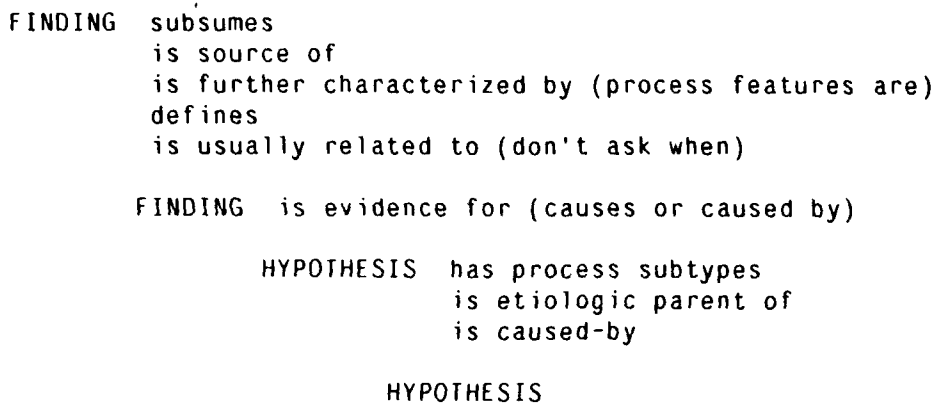
Figure 4-3: Summary of basic domain relations in NEOMYCIN.
