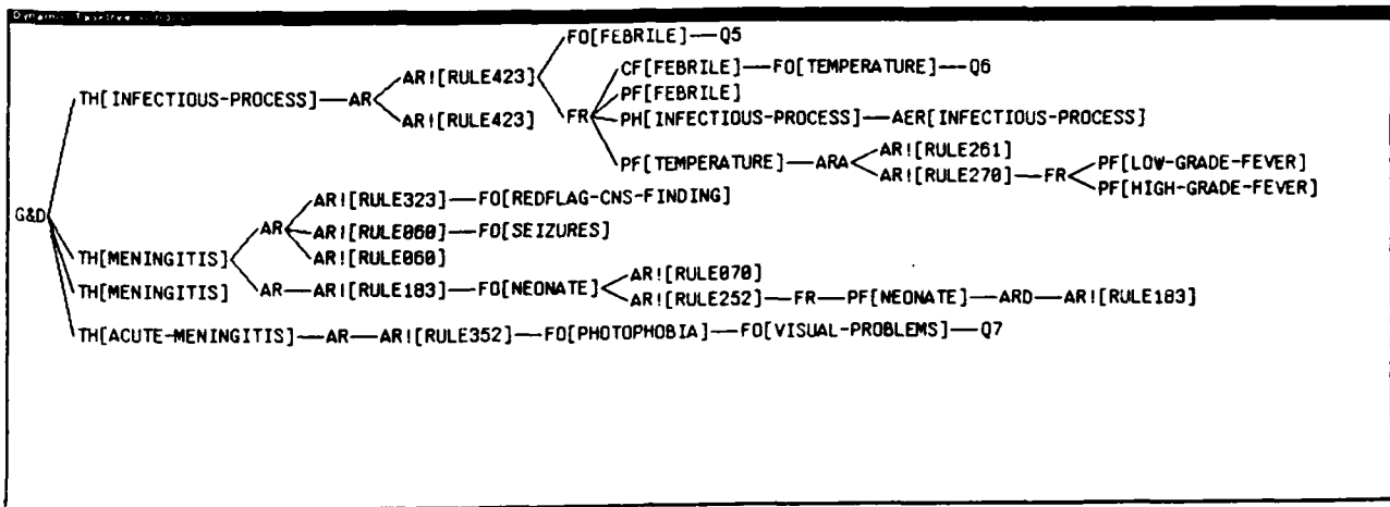
Figure 4-14: The Dynamic Task Tree Window.
