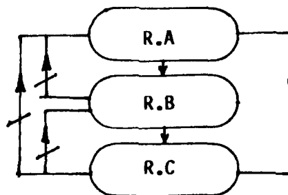
Figure 3.2.3 Transitive Dependence
