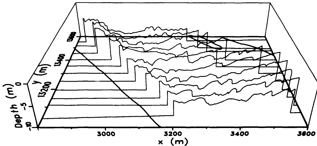
FIGURE 19 Perspective Plot of Transverse Bathymetric Transects for Survey IX at the Gordon's Ferry Disposal Site
