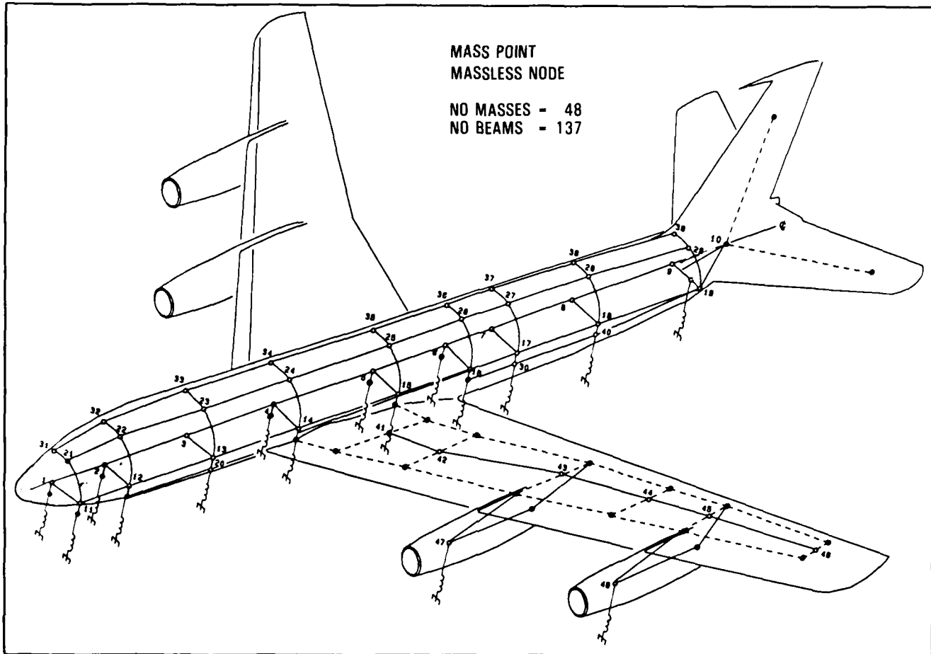
FIGURE 18. EXPANDED CID MODEL (REFERENCE 20)
