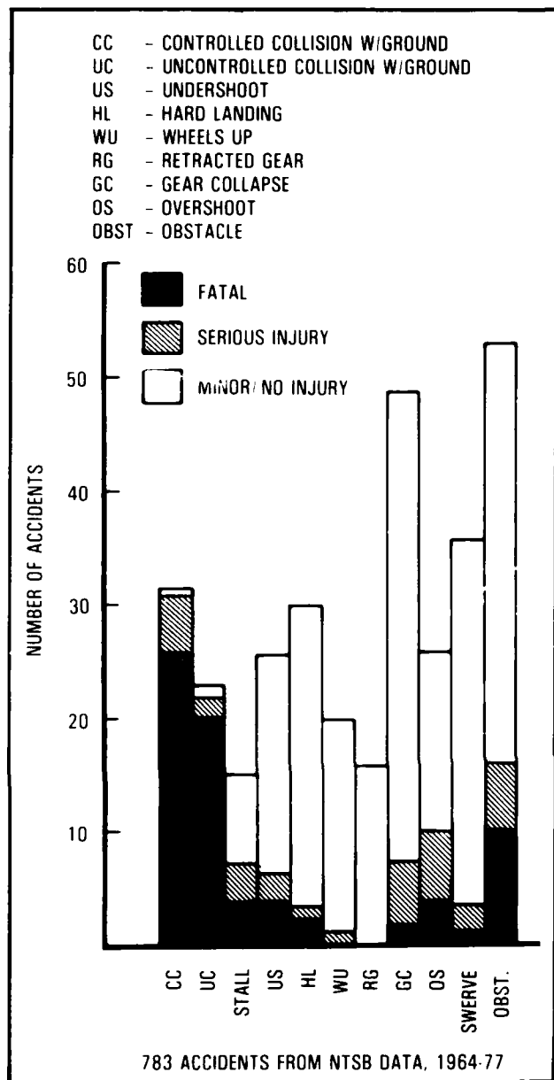
FIGURE 4. SUMMARY OF RESULTS OF ACCIDENT STUDY (REFERENCE 4)
