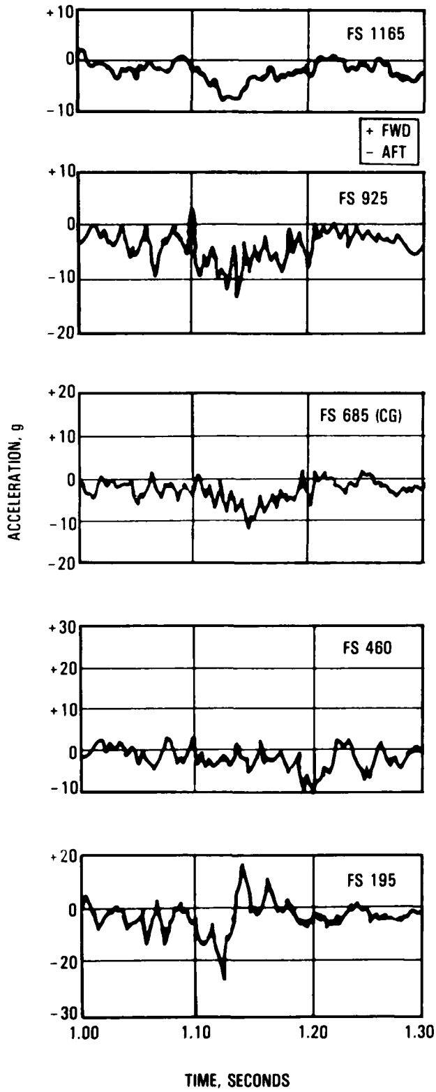
FIGURE 5. FLOOR LONGITUDINAL ACCELERATIONS, L-1649 TEST, 6-DEGREE SLOPE IMPACT (REFERENCE 8)
