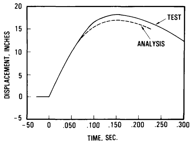
(a) VERTICAL DISPLACEMENT VERSUS TIME
