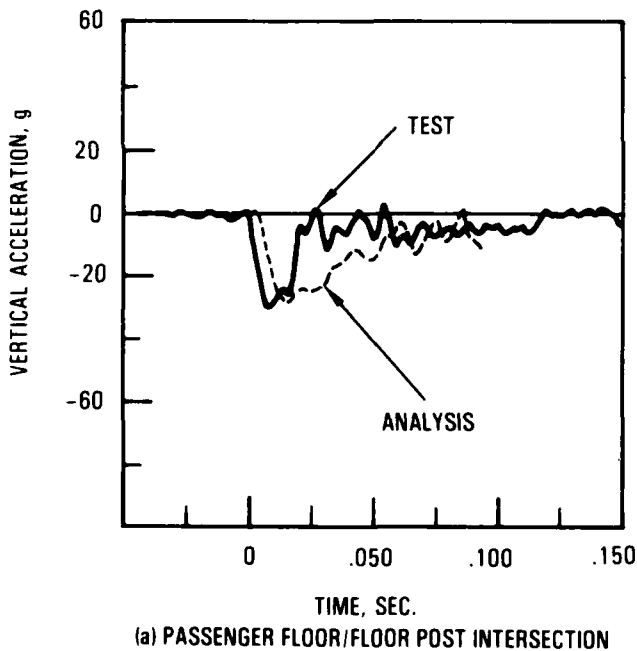
FIGURE 17. COMPARISON OF WIDEBODY FRAME SECTION ANALYSIS AND TEST RESULTS (REFERENCE 20)
