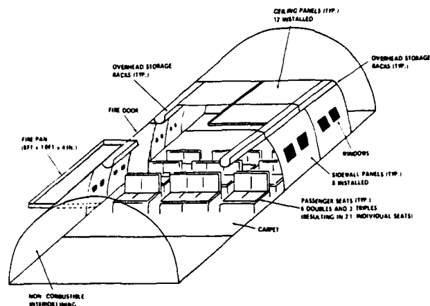
Figure 2. Installation of Wide-Body Materials Inside C-133 Test Article
