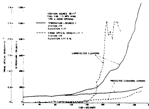
Figure 11. Seat Cushion Blocking Layer Benefit — Postcrash Fuel Fire Adjacent to Open Door
