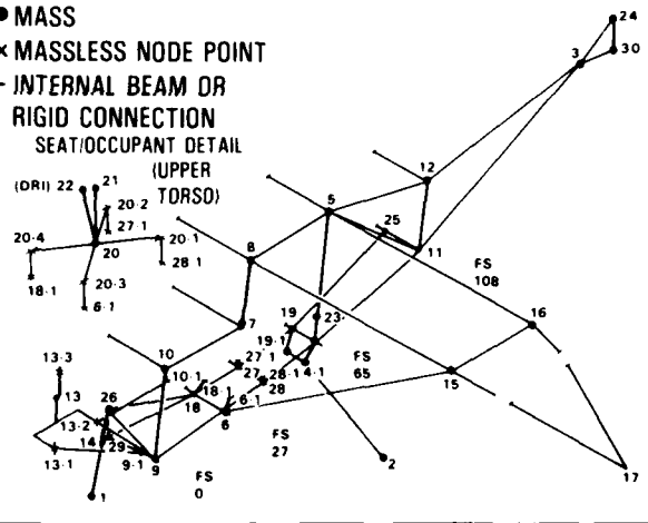
FIGURE 12. SINGLE-ENGINE HIGH-WING AIRPLANE ANALYTICAL MODEL (REFERENCE 14)
