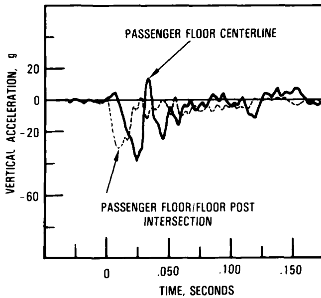
FIGURE 10. RESULTS OF WIDE-BODY AIRPLANE AFT FUSELAGE SECTION TEST (REFERENCE 12)
