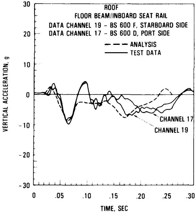
(a) FLOOR BEAM/INBOARD SEAT RAIL
