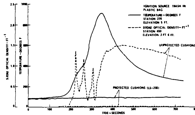
Figure 3. Seat Cushion Blocking Layer Benefit — Ramp Fire Scenario
