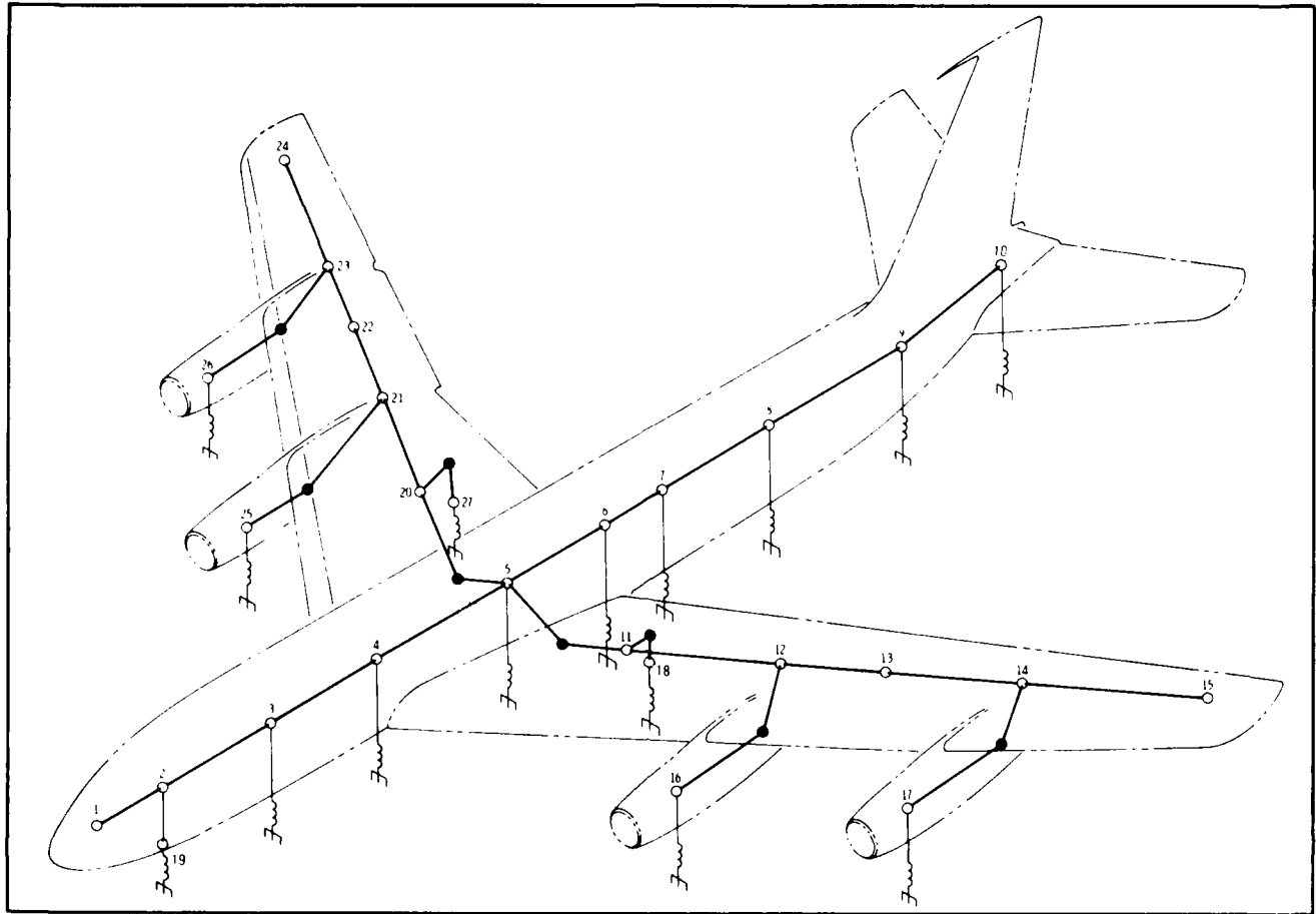
FIGURE 19. CID STICK MODEL (REFERENCE 20)
