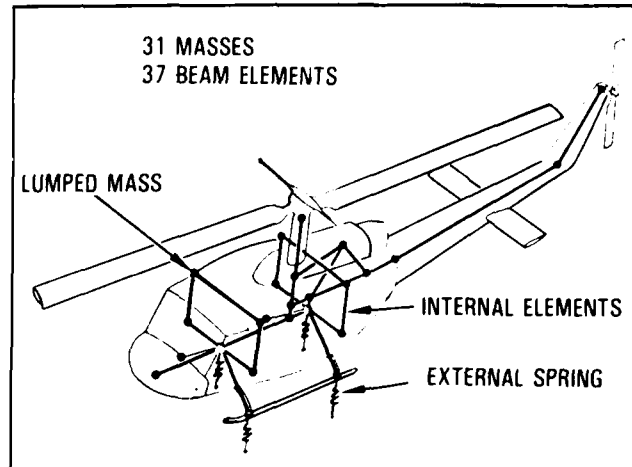
FIGURE 11. HELICOPTER ANALYTICAL MODEL (REFERENCE 13)
