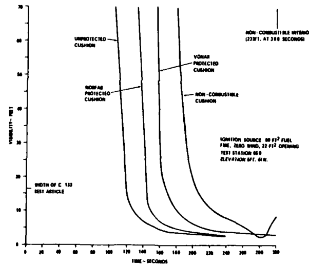
Figure 9. Effect of Cushioning Protection on Calculated Visibility Through Smoke Under Full-Scale Postcrash Fire Conditions
