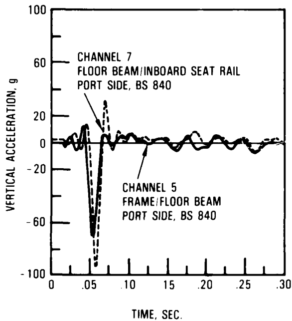
FIGURE 8. RESULTS OF NARROW-BODY AIRPLANE FUSELAGE CENTER SECTION TEST (REFERENCE 10)
