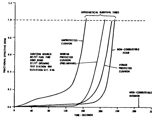
Figure 8. Effect of Cushioning Protection on Calculated Survival Time Under Full-Scale Postcrash Fire Conditions
