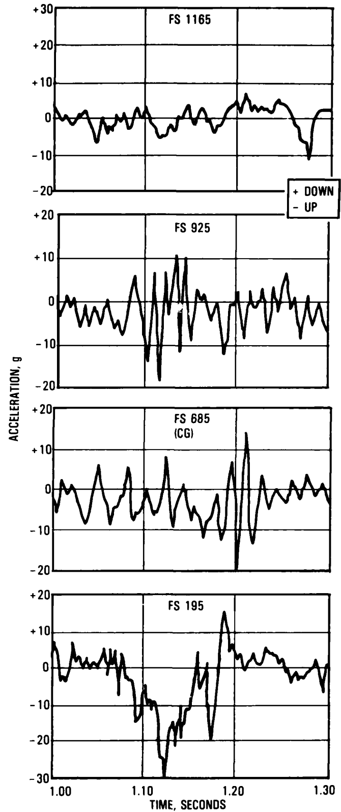
FIGURE 6. FLOOR VERTICAL ACCELERATIONS, L-1649 TEST, 6-DEGREE SLOPE IMPACT (REFERENCE 8)
