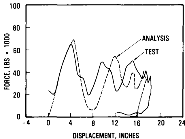
(b) FORCE VERSUS DISPLACEMENT, VERTICAL
