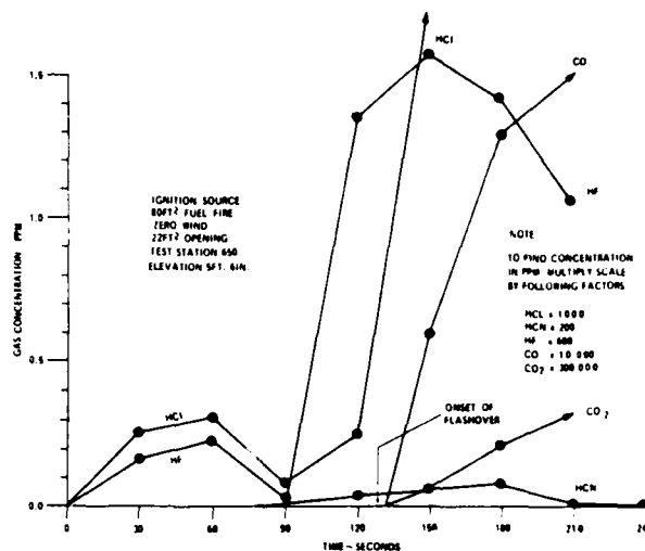
(b) During a Postcrash Fire
