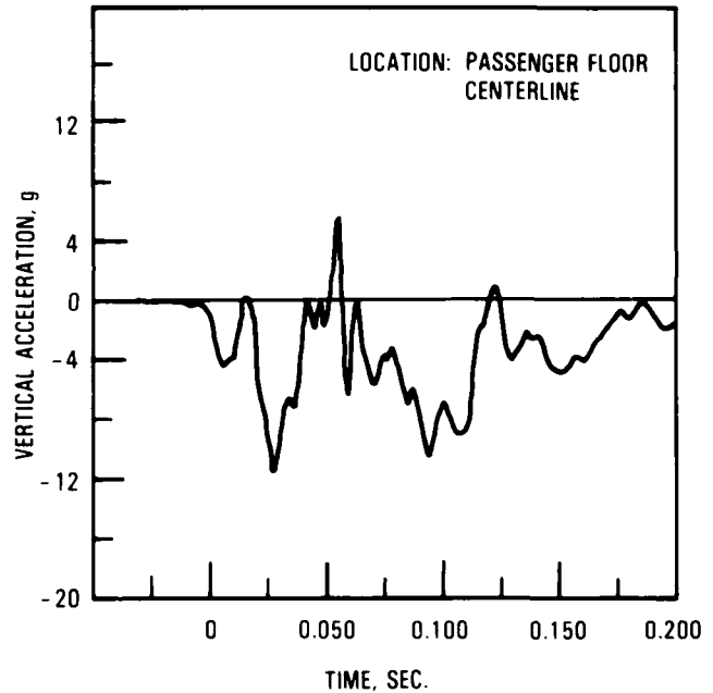
FIGURE 9. RESULTS OF NARROW-BODY AIRPLANE FORWARD FUSELAGE SECTION (WITH CARGO) TEST (REFERENCE 11)
