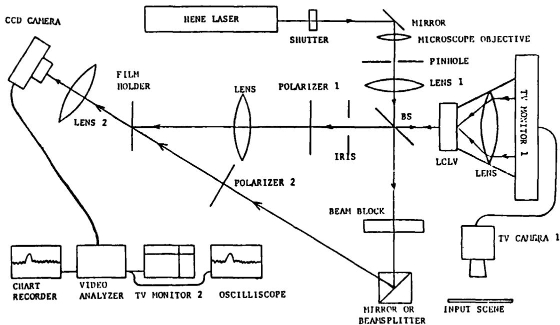
Figure 2. The real-time optical correlator - experimental arrangement.
