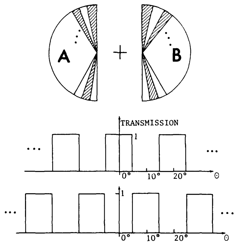
Figure 6. The transmission function for the "phase shifted" Ronchi ruling.
