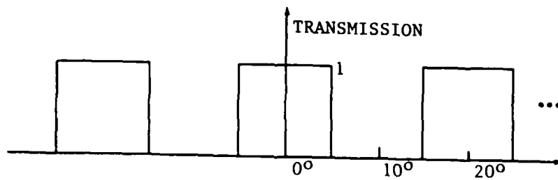
Figure 4. The transmission function for the angular Ronchi ruling.
