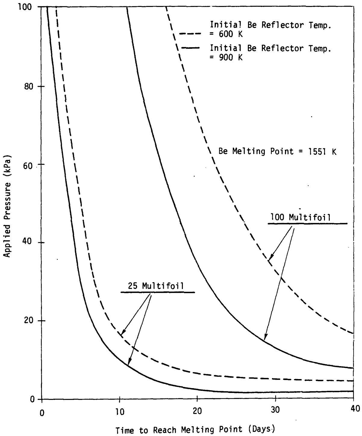
Figure 36. Applied pressure.
