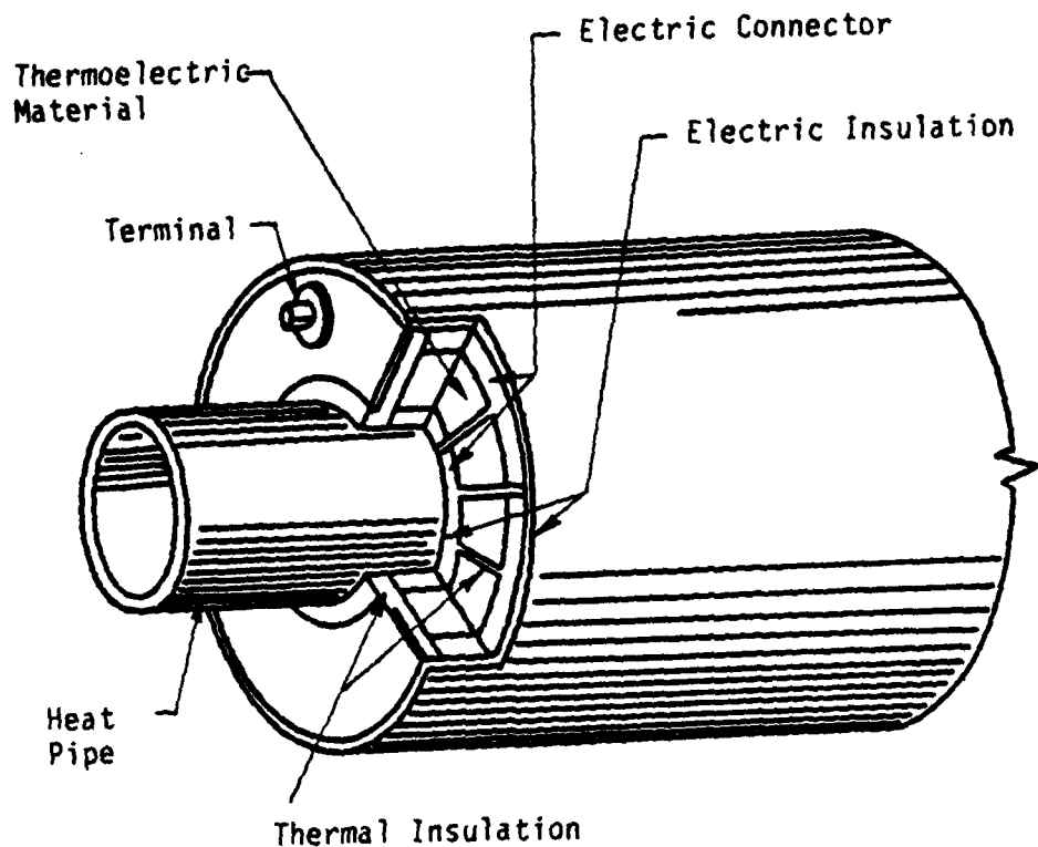
Figure B-9. Thermoelectric module (Ref. 1).
