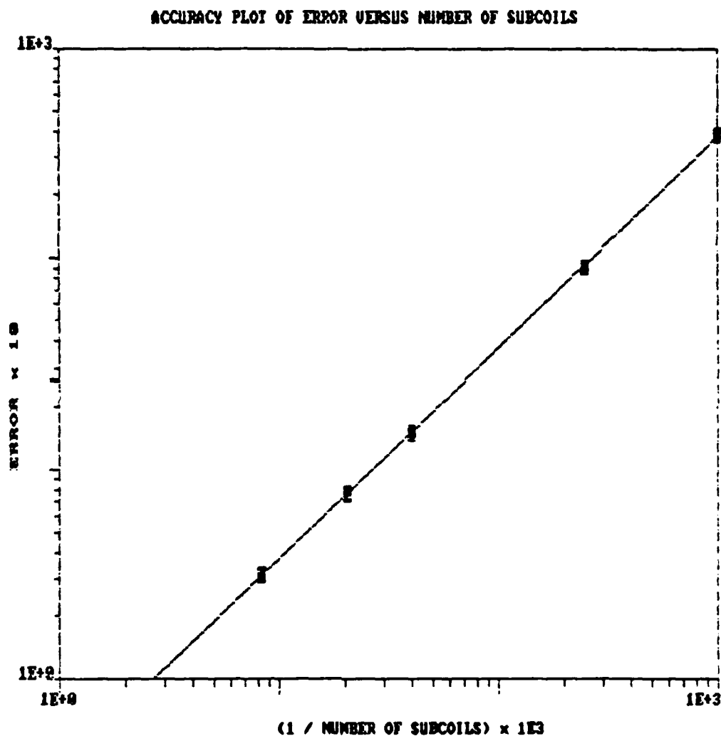
Figure 5.3: A Log/Log Accuracy Plot of Self Inductance
