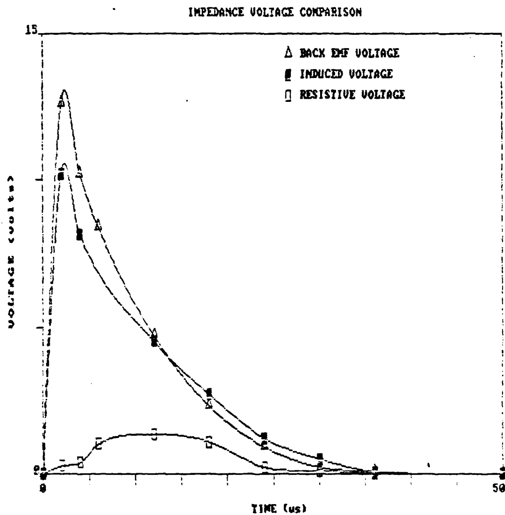
Figure 6.9: Voltage Parameter Comparison
