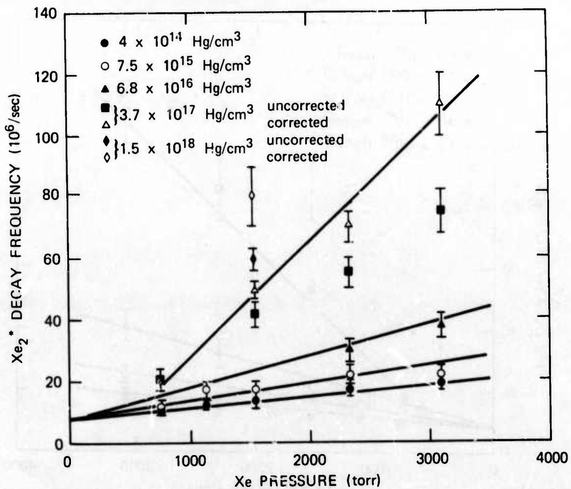
FIGURE 12 Xe_2^* (1720Å) DECAY FREQUENCY VERSUS Xe PRESSURE FOR VARIOUS Hg DENSITIES
