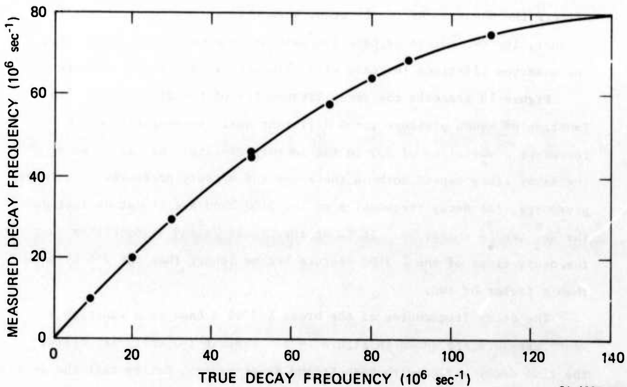
FIGURE 10 EFFECT OF SODIUM SALICYLATE RADIATIVE LIFETIME ( \tau_R = 12 \text{ ns} ) ON MEASURED DECAY FREQUENCIES
