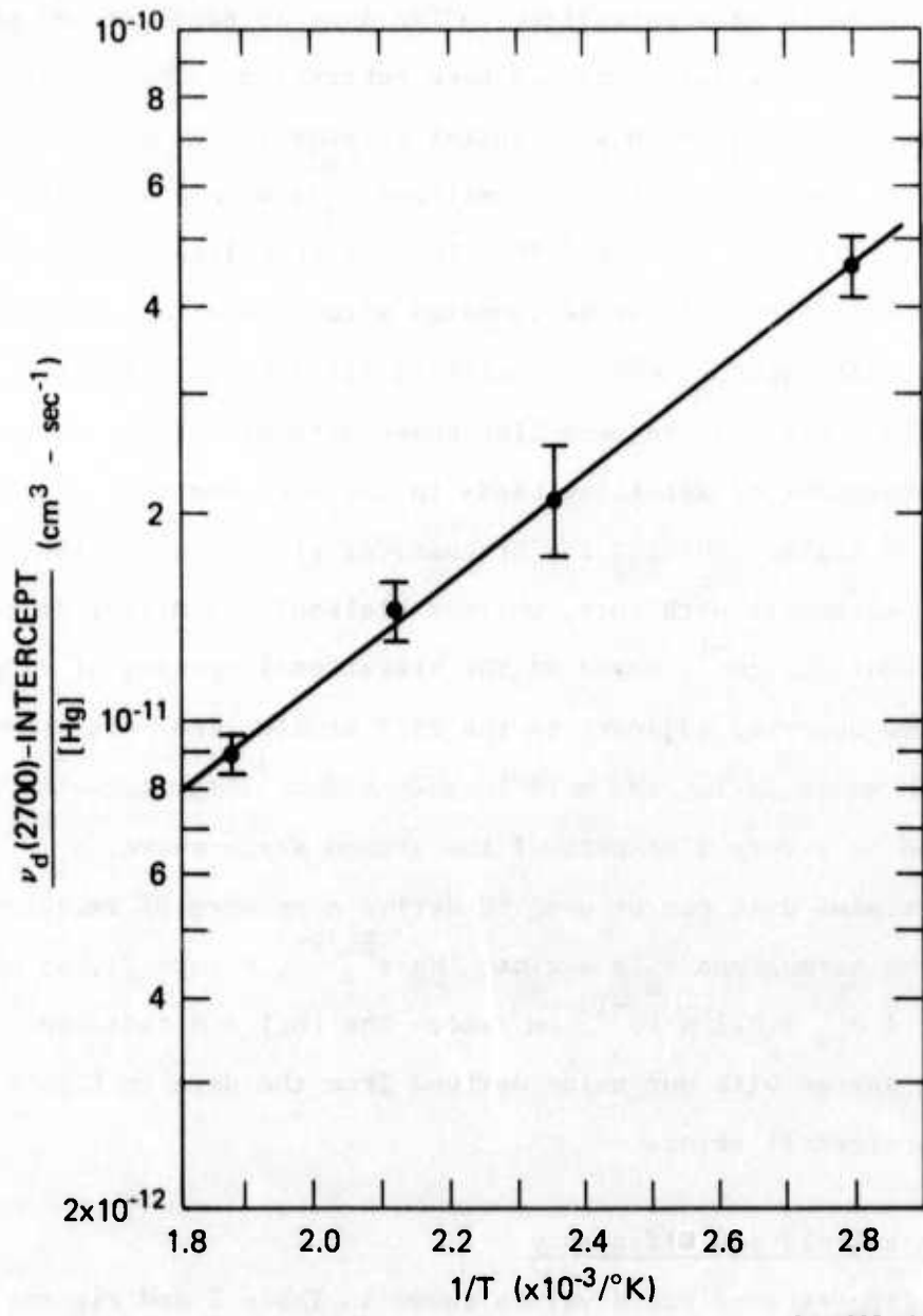
FIGURE 20 EFFECTIVE WELL DEPTH CALCULATION The quantity subtracted from \nu_d(2700) is the intercept value at zero xenon pressure. The slope yields 1300 \text{ cm}^{-1} .
