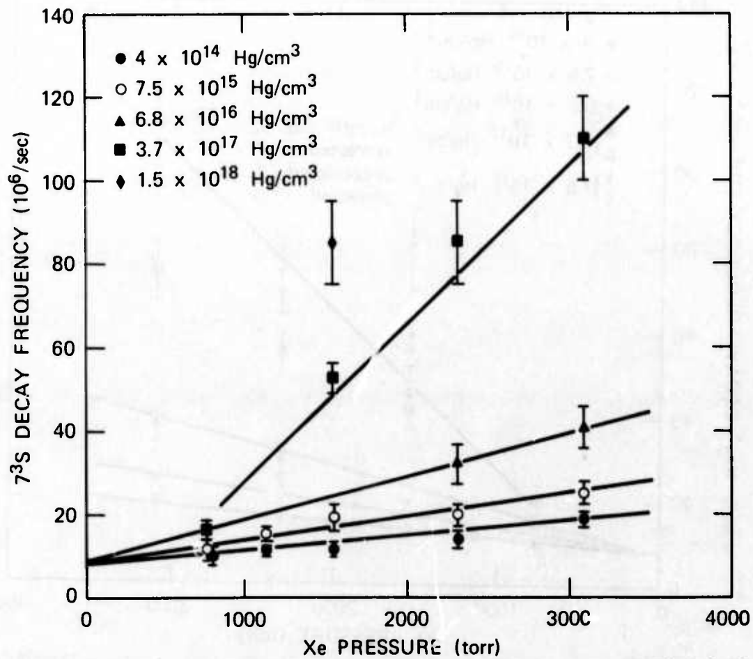
FIGURE 11 Xe-Hg ( 7^3S ) DECAY FREQUENCY VERSUS XE PRESSURE FOR VARIOUS Hg DENSITIES
