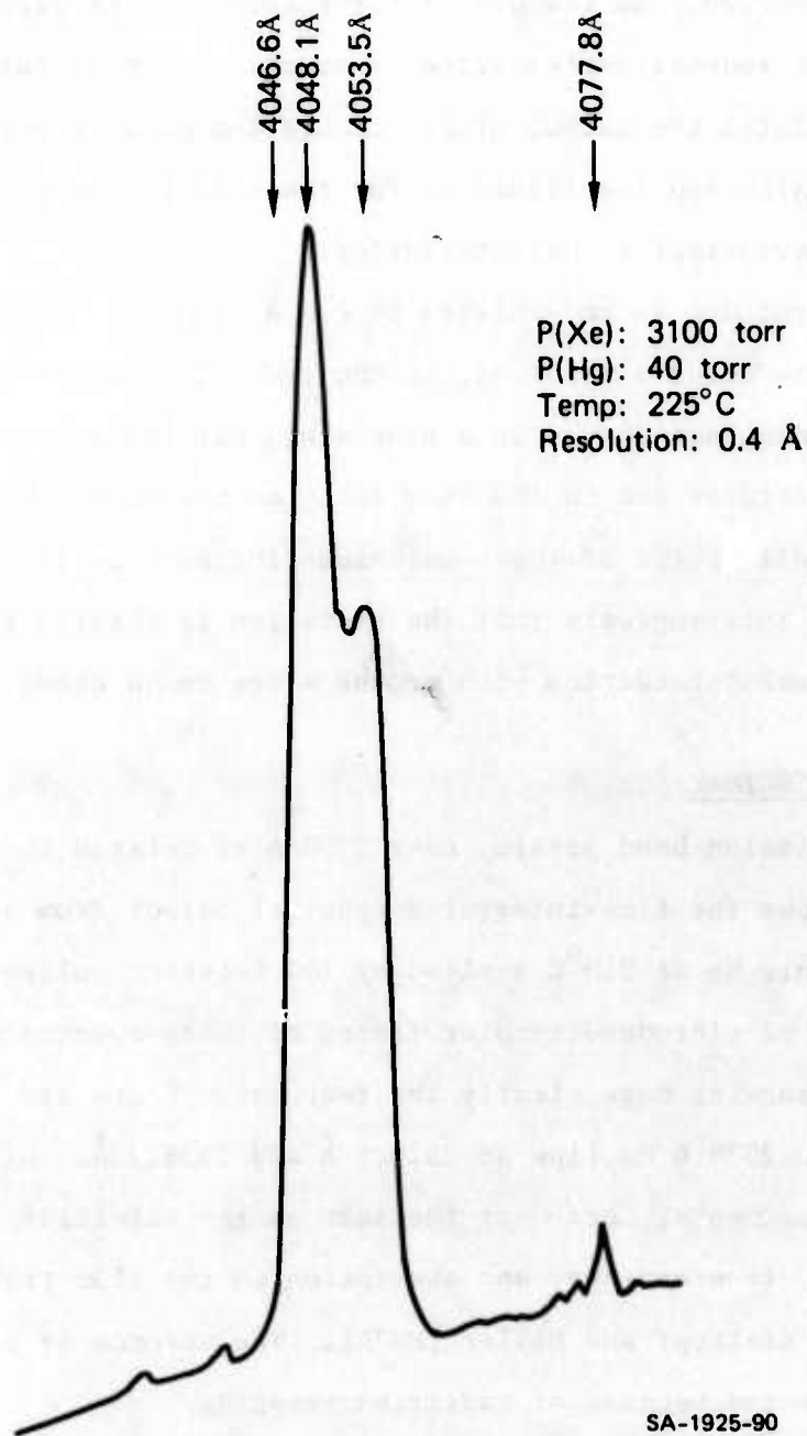
FIGURE 4 MICRODENSITOMETER TRACING OF THE PERTURBED Hg ( 7^3S-6^3P_0 ) EMISSION
