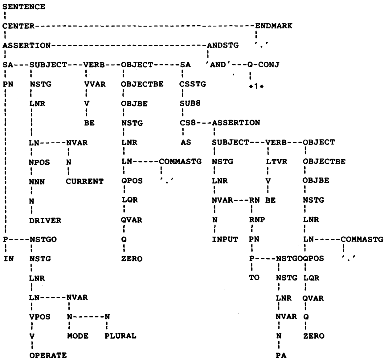
Fig. 3 — Regularized parse tree
