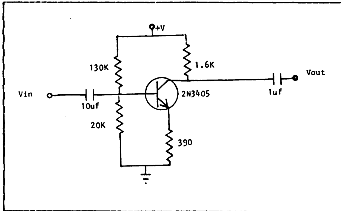
Figure 4.1 Common-Emitter Amplifier.
