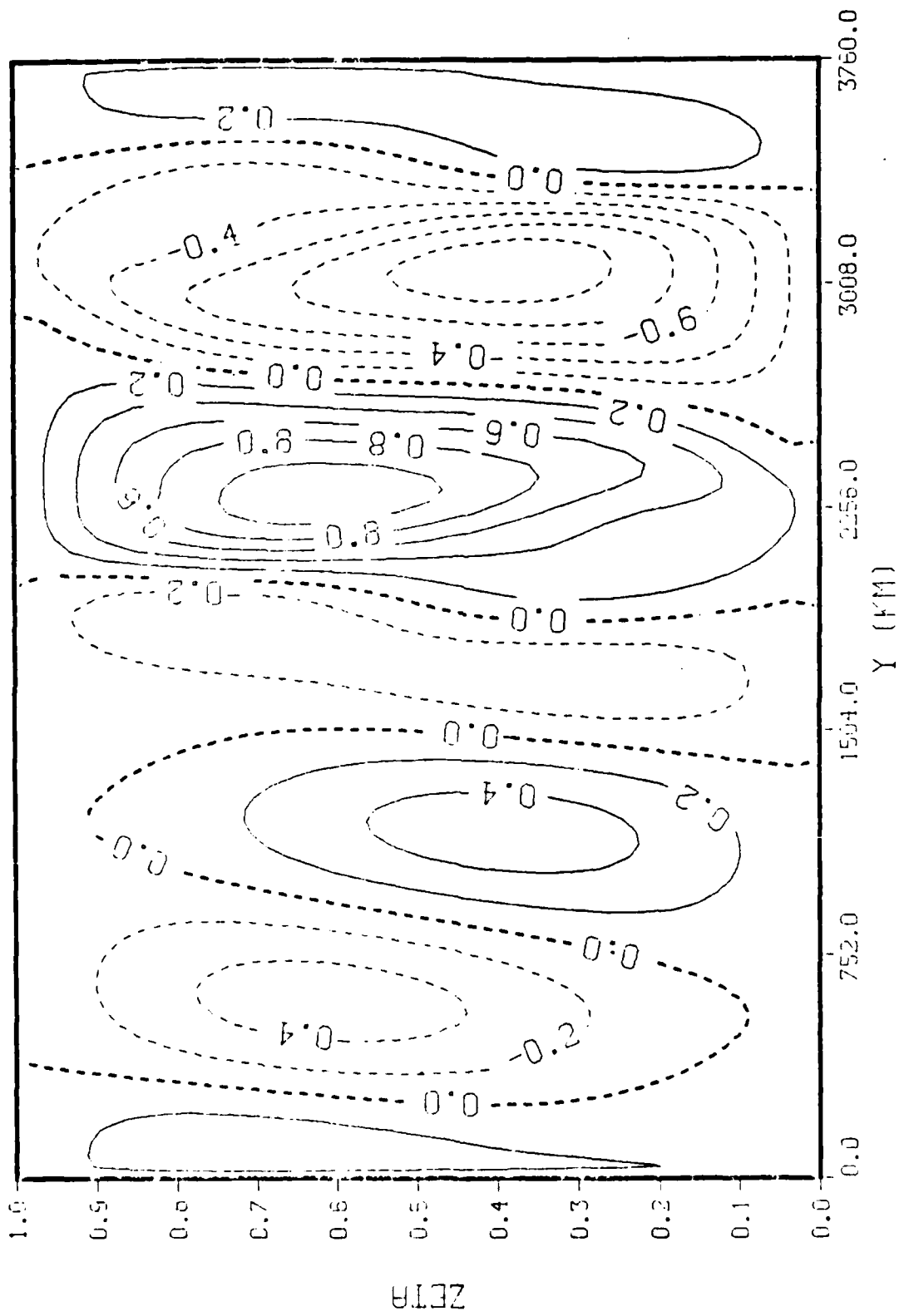
Fig. 19. \dot{\epsilon} ( \times 10^{-6} \text{ sec}^{-1} ). 24 hours. Deformation only
