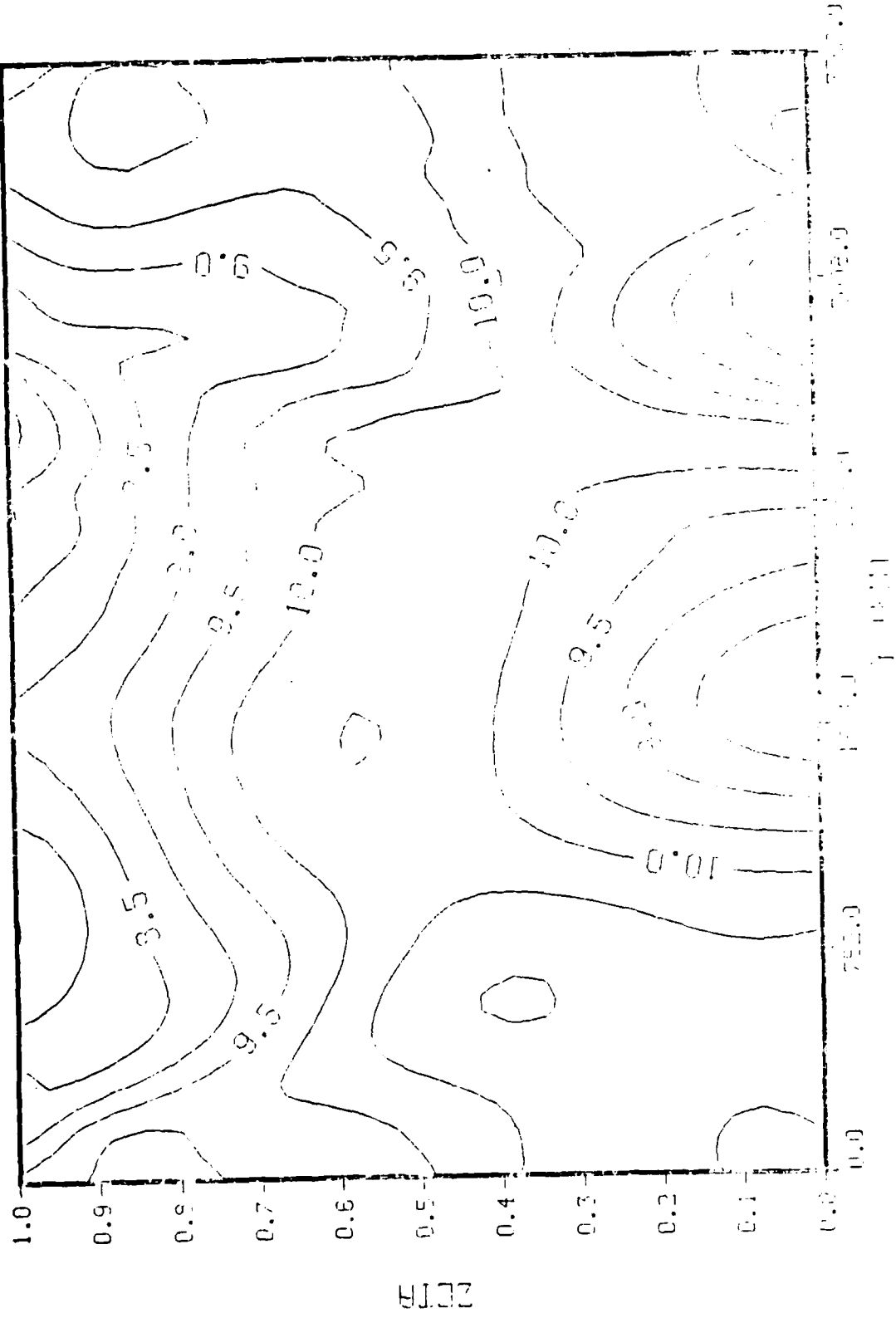
Fig. 32. v (m/sec). 46 hours. Deformation and mountain
