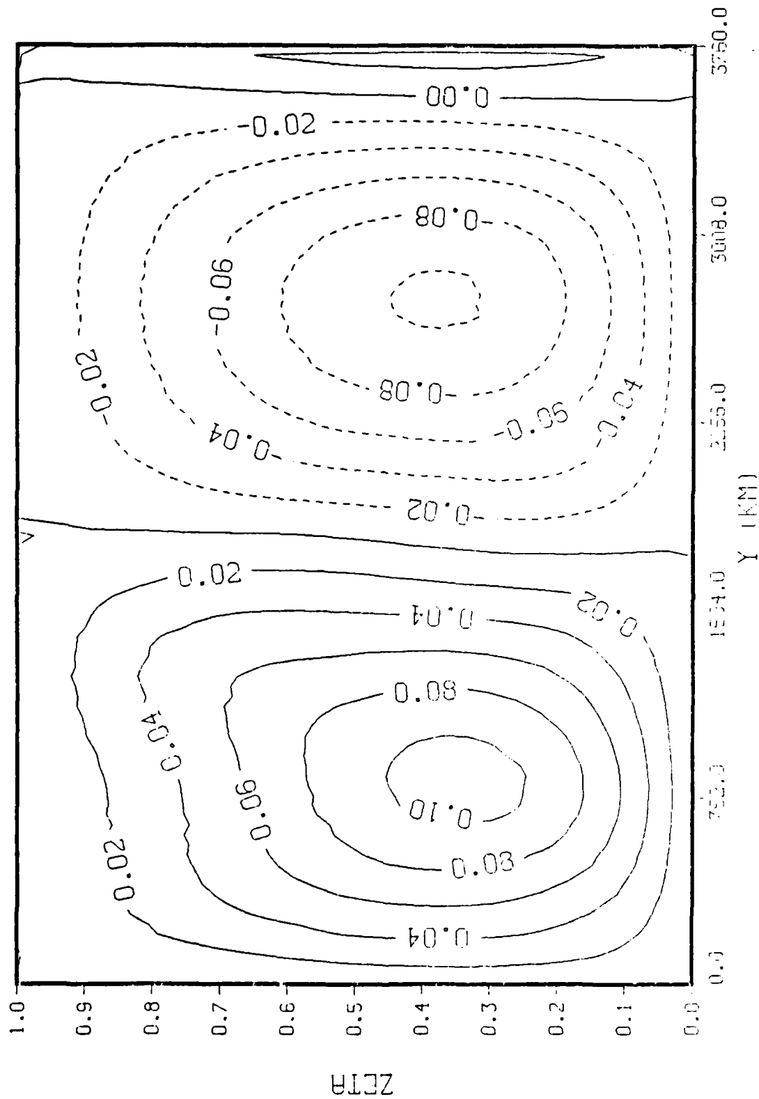
Fig. 12. \xi ( \times 10^{-6} \text{ sec}^{-1} ). 72 hours. Mountain only
