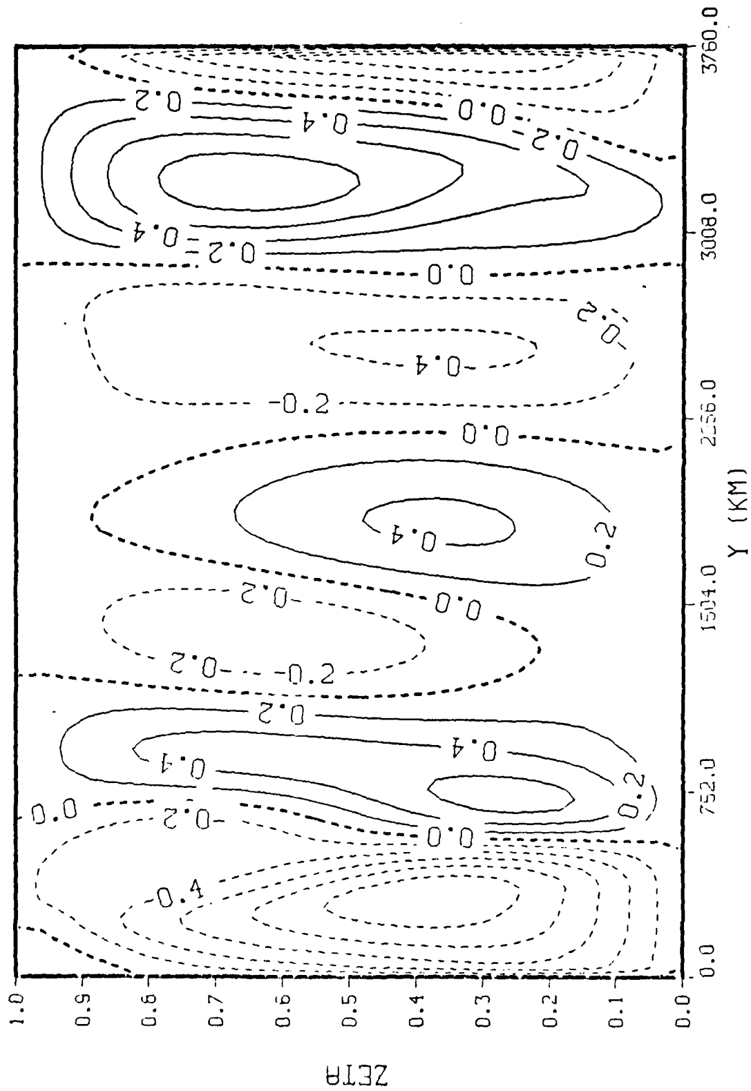
Fig. 37. \dot{\xi} ( \times 10^{-6} \text{ sec}^{-1} ). 24 hours. Maximum deformation over valley
