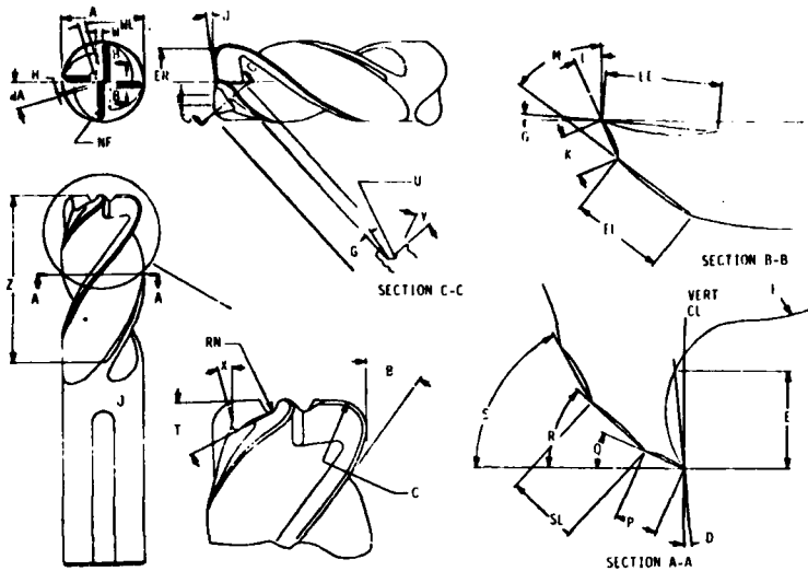
Figure 2 - Cutter Geometry
