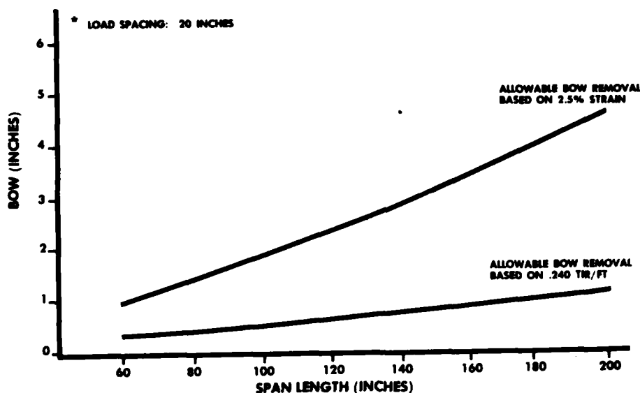
Figure 1 - VS Span Length for 155mm M185
