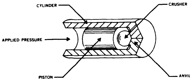
Figure 1 - Copper Crusher Pressure Gage
