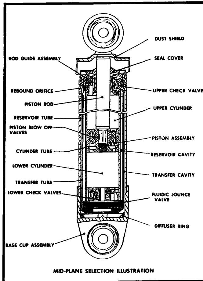
Figure 1 - Fluidic Damper
