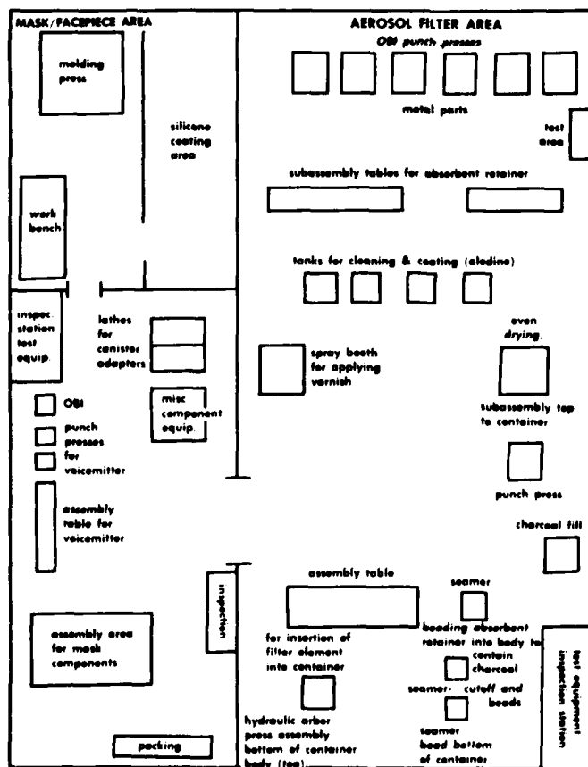
Figure 1 - P-T Line - XM30 New Protective Mask
