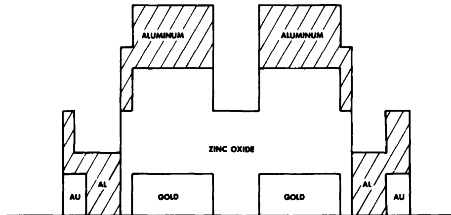
Figure 1 - ZnO Transducer Cross Section
