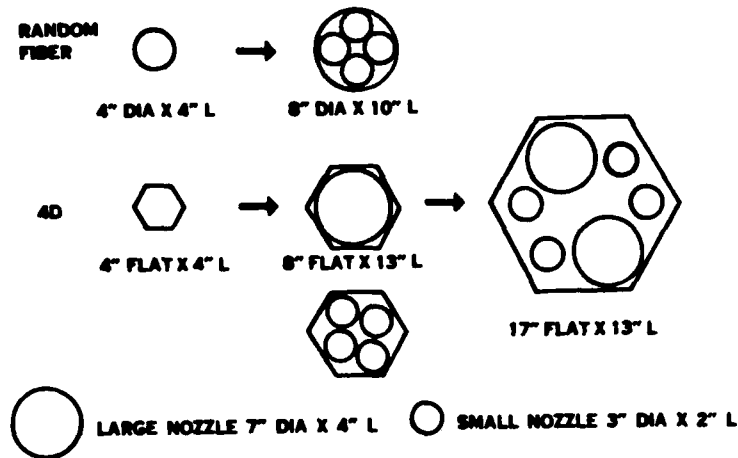
Figure 1 - Carbon-Carbon Billet Configurations
