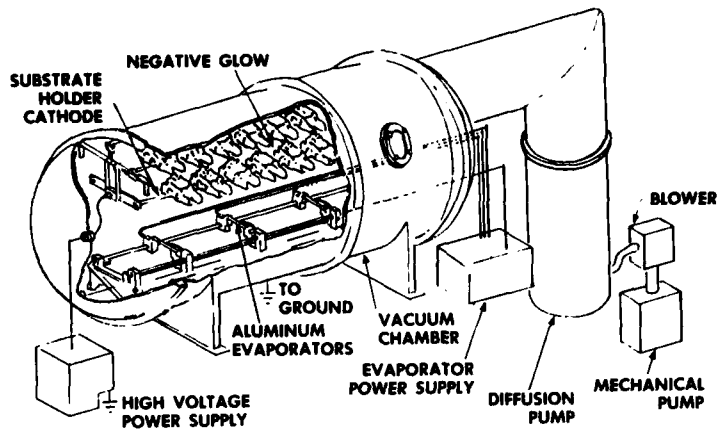
Figure 1 - Schematic of an Ion Vapor Deposition System
