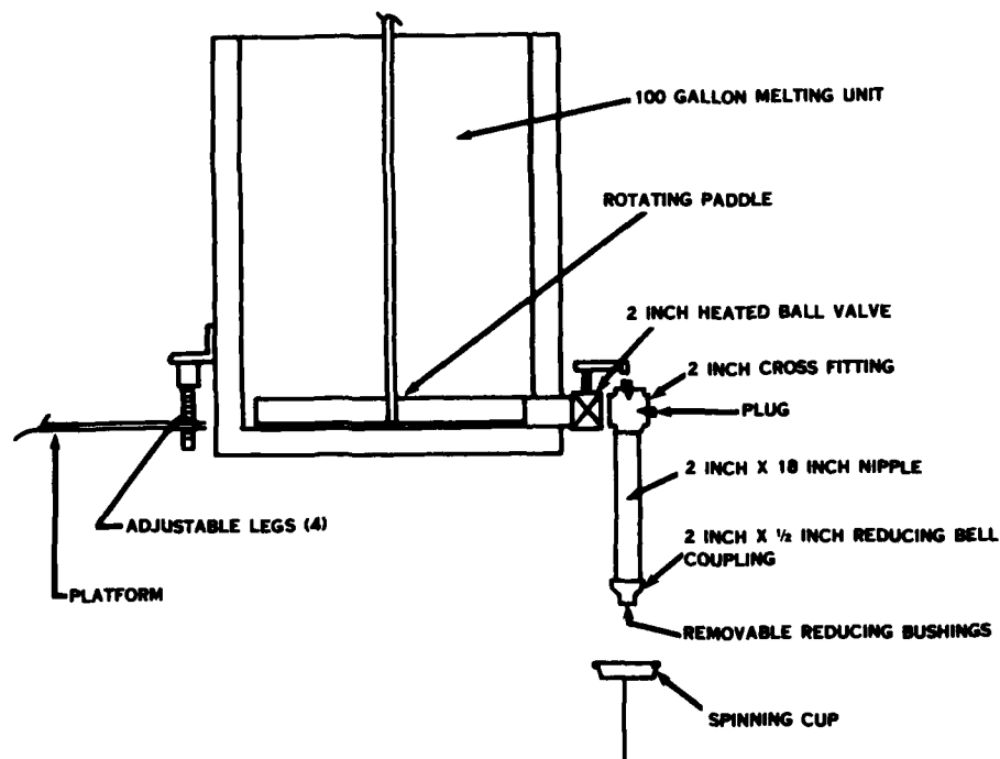
Figure 1 - Melting Container and Spinning Cup
