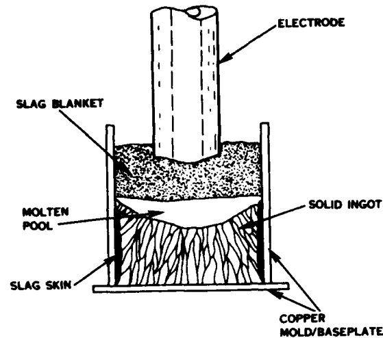
Figure 1 - ESR Process
