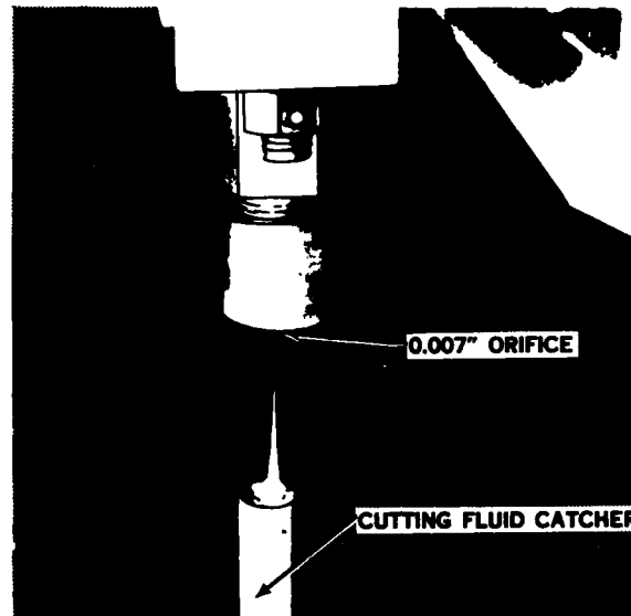
Figure 1 - Fluid Jet Cutter
