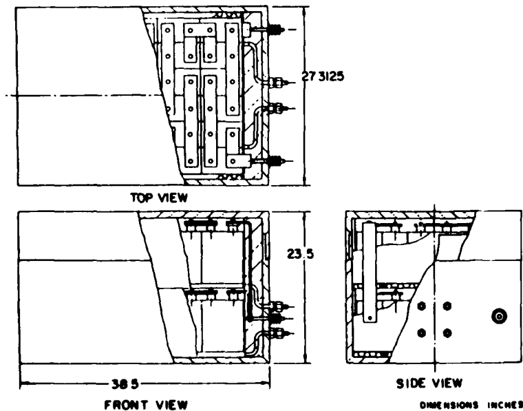
Figure 1 - Battery Layout
