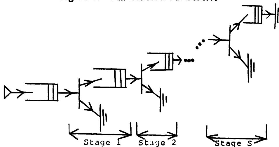
Figure 6: Non-full tree
