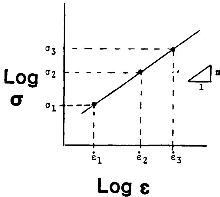
Figure 4.11 Schematic diagrams illustrating determination of m : a) true stress vs. true strain for various strain rates; b) \log \sigma vs. \log \epsilon , with \sigma = B\epsilon^m , m = slope.
