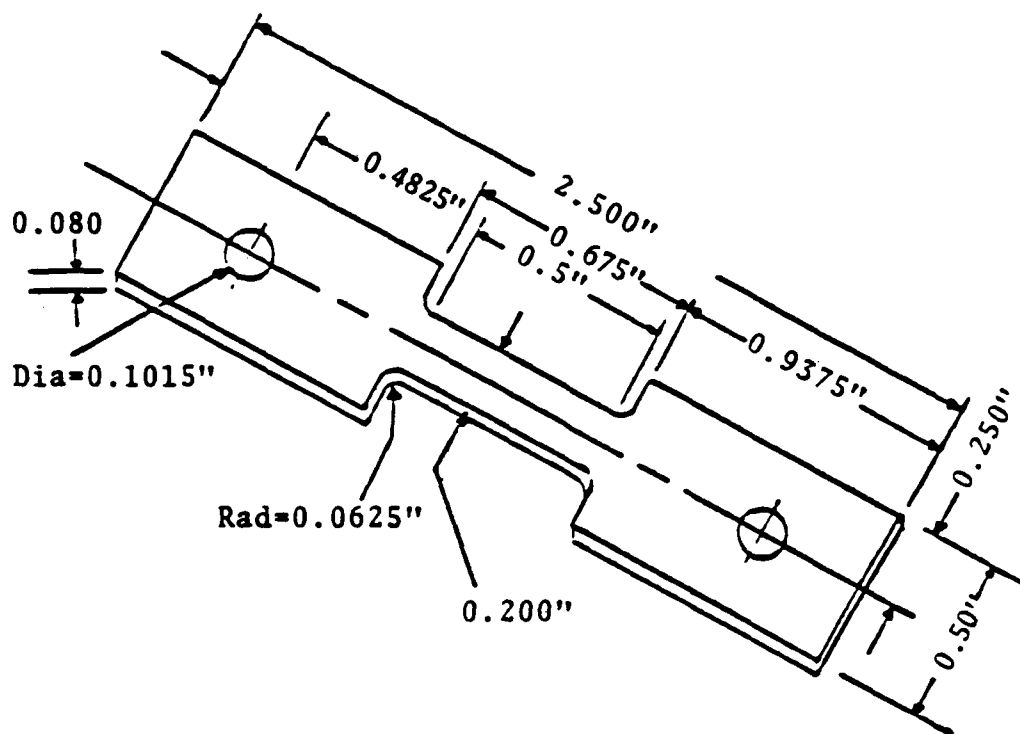
Figure 3.4 New specimen geometry.
