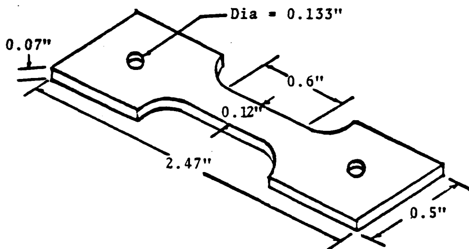
Figure 3.3 Old specimen geometry.
