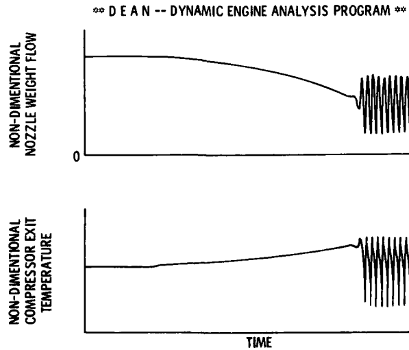
Figure 7. - Time traces of weight flow and temperature.
