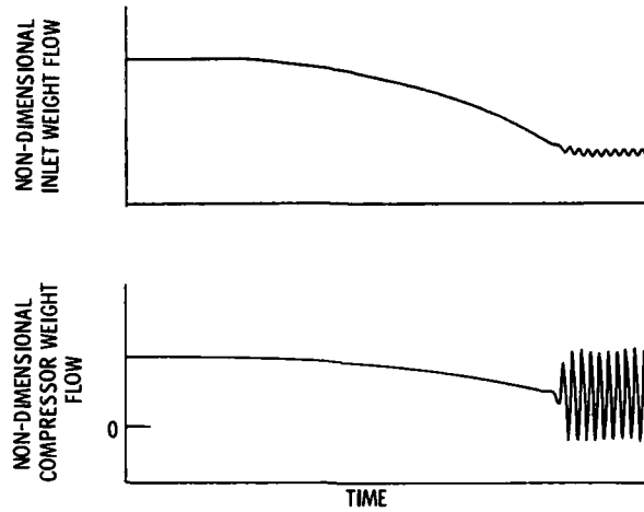
Figure 6. - Time traces of weight flow.
