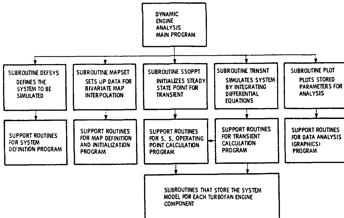
Figure 1. - Simplified diagram of Dean subroutines.
