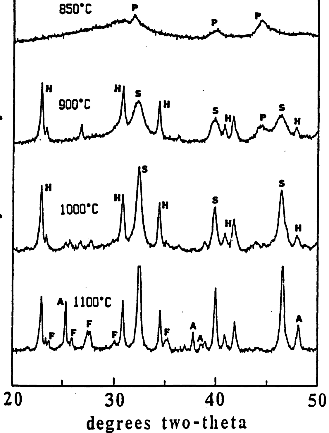
Figure 1. XRD patterns of SAR-2-P glass-ceramics, crystallized at various temperatures for one hour. Phases indicated as: P) precursor phase and S) perovskite \text{SrTiO}_3 ; H) hexacelsian and anorthite \text{SrAl}_2\text{Si}_2\text{O}_8 ; A) anatase \text{TiO}_2 .
