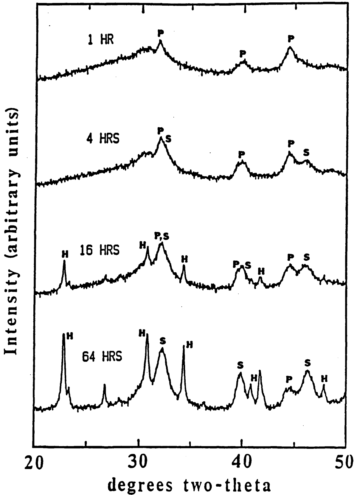
Figure 2. XRD patterns of SAR-2-P glass-ceramics, crystallized at 850°C for various times. Phases indicated as: P) precursor phase and S) perovskite SrTiO 3 ; H) hexacelsian SrAl 2 Si 2 O 8 .
