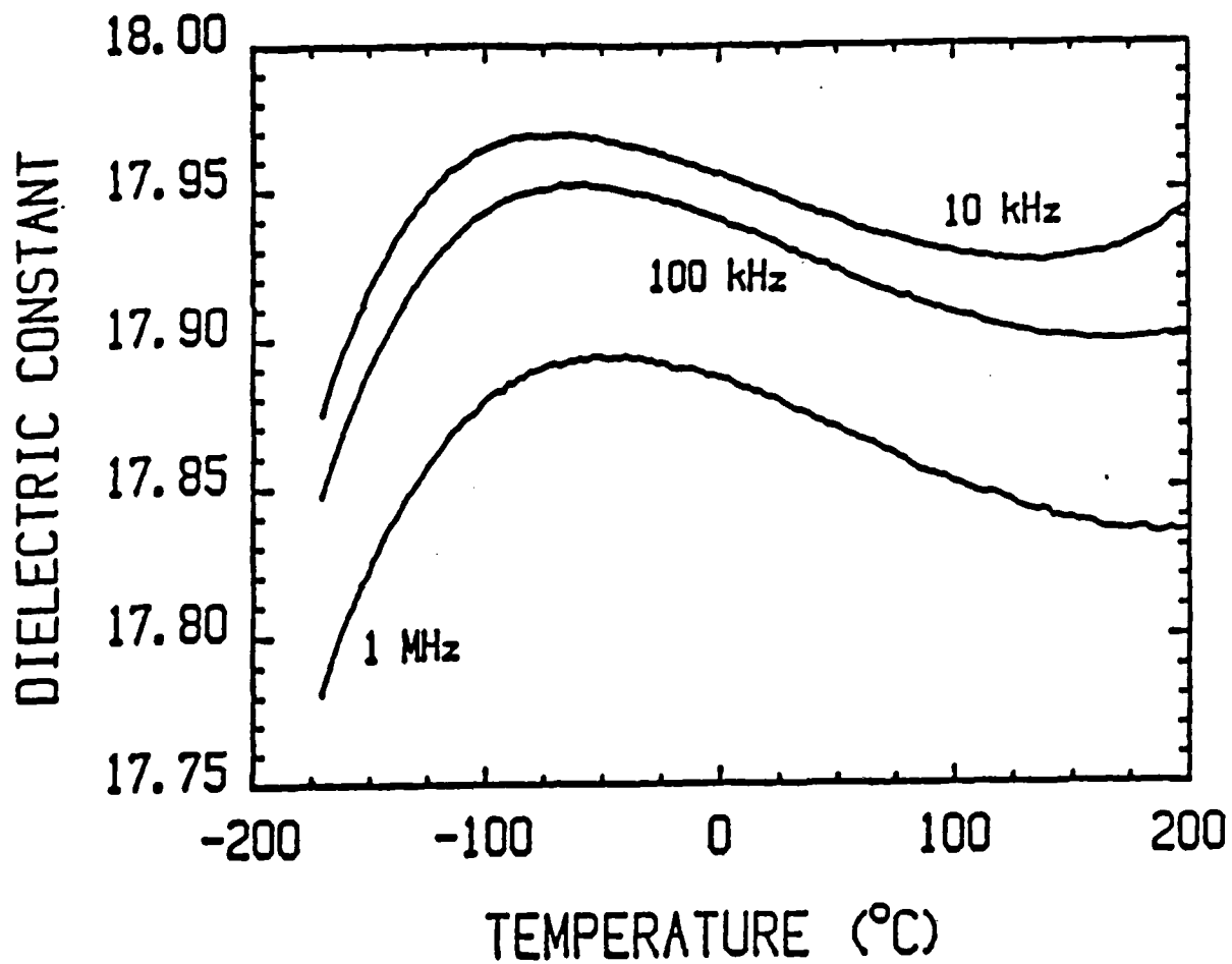
Figure 3. Dielectric constant at 10, 100, and 1000 kHz versus temperature, for the SAR-2-P glass-ceramic, conventionally crystallized at 842°C for one hour.
