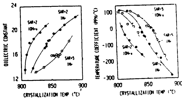
FIGURE 2 a) Dielectric constant and b) temperature coefficient vs. crystallization temperature for various glass compositions and crystallization conditions.
