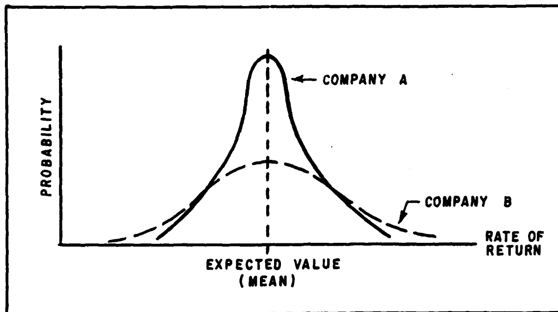
FIGURE 5-1. RISK-RETURN CONCEPT
