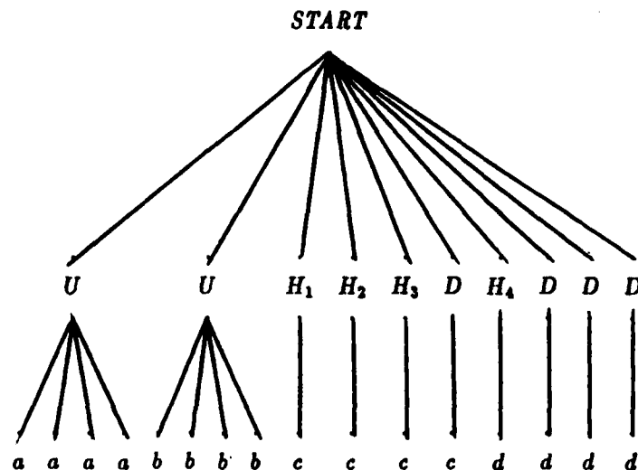
Figure 4: The grammar of Figure 3, which encodes the vertex-cover problem of Figure 2, generates the string \sigma = aaaabbbbccccdddd according to this parse tree. The vertex cover \{c, d\} can be read off from the parse tree as the set of elements dominated by H -symbols.
