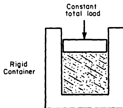
Figure F1. Idealization of vertical deformation with lateral restraint (uniaxial compression test)
