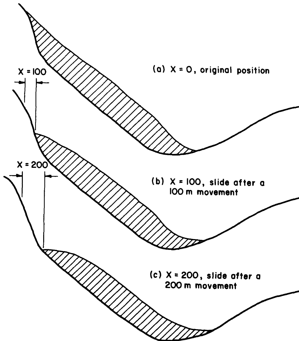
Figure E1. Slide at Various Stages of Movement
