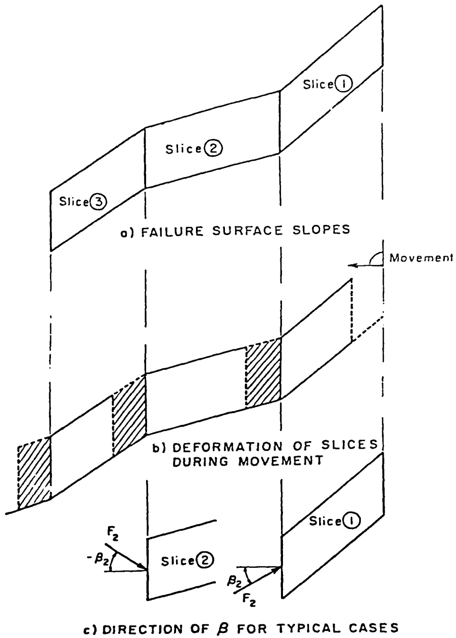
Figure B3. Illustration of method for assigning direction of frictional forces between slices
