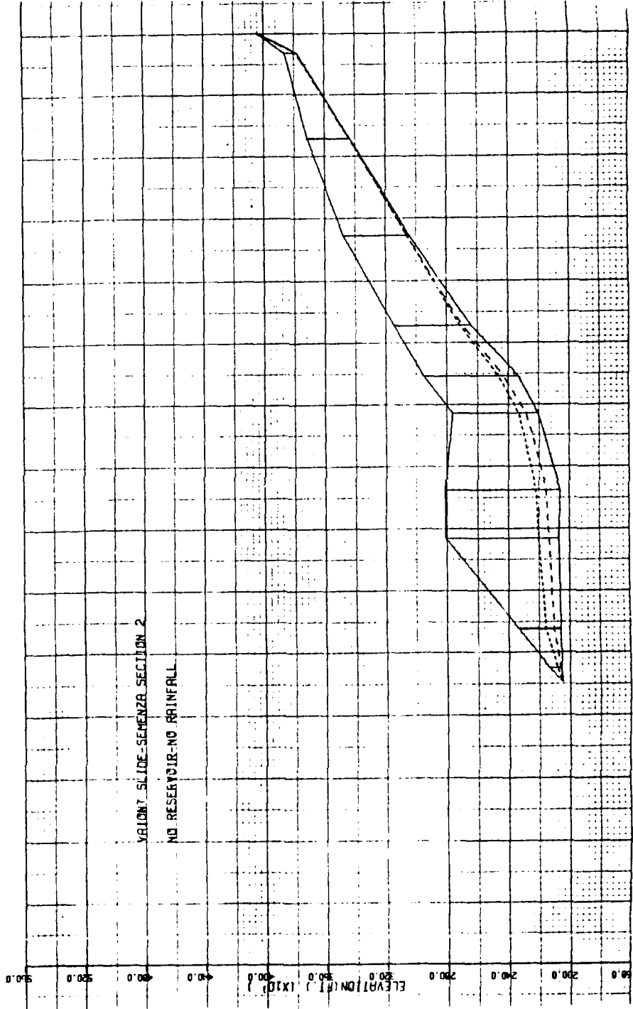
Figure C1. Vaiont Slide - Semenza Section 2, No reservoir, no rainfall
