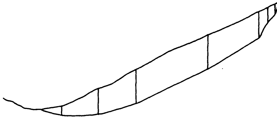
Figure B1. Subdivision of slide into slices
