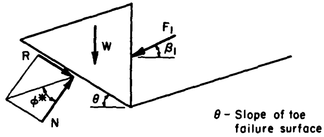
a) Forces on toe wedge
