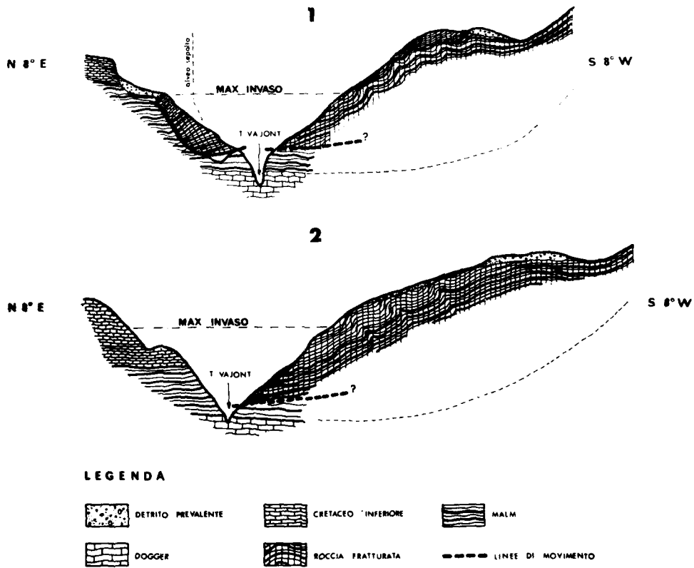
Figure G3. Geological profiles of the "Pian del Toc" zone, taken from the Geological Study of the Vaiont Reservoir" by F. Giudici and E. Semenza, 1960. (See note, Fig. G2)
