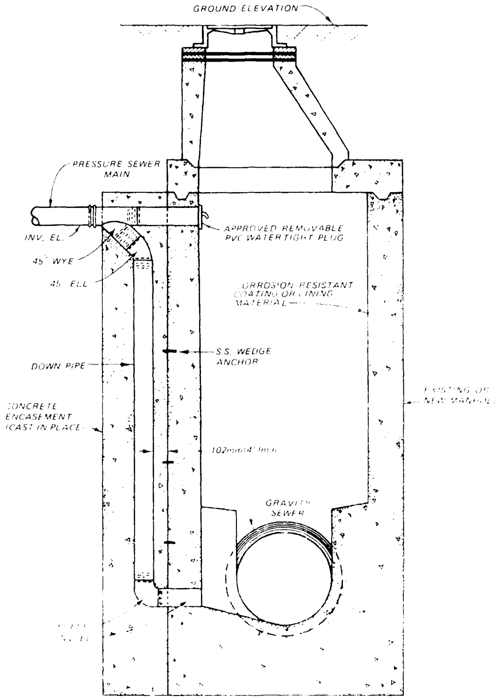
FIGURE 22. DETAIL FOR PRESSURE MAIN CONNECTION
