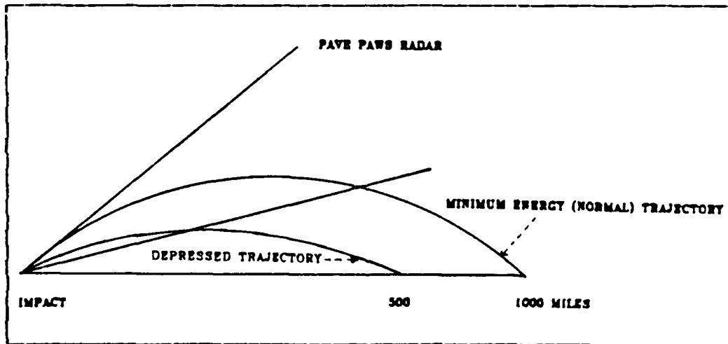
Figure 3.9 Two Possible SLBM Trajectories
