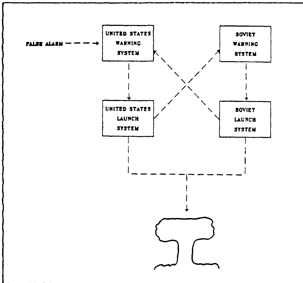
Figure 2.2 The Bereanu Model
