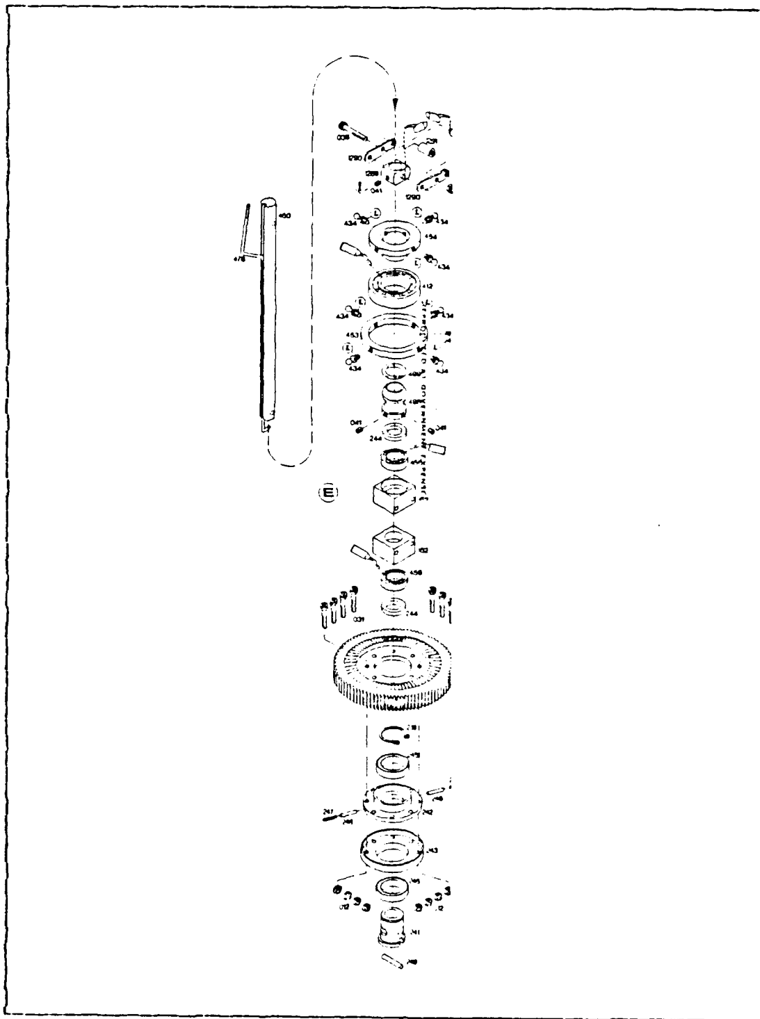
Figure A.3 Main Rotor Drive Gear & Swash Plate Assembly
