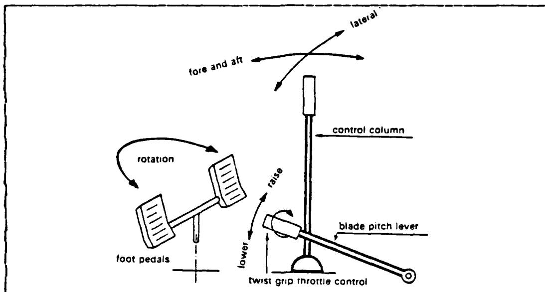
Figure 3.1 Full-size Helicopter Control Arrangement
