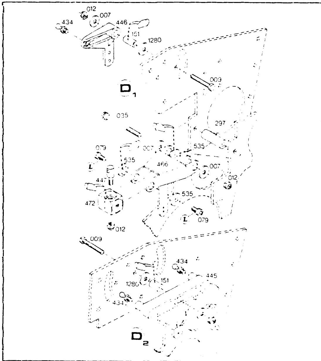
Figure A.1 Lateral & Longitudinal Cyclic Lever Assembly
