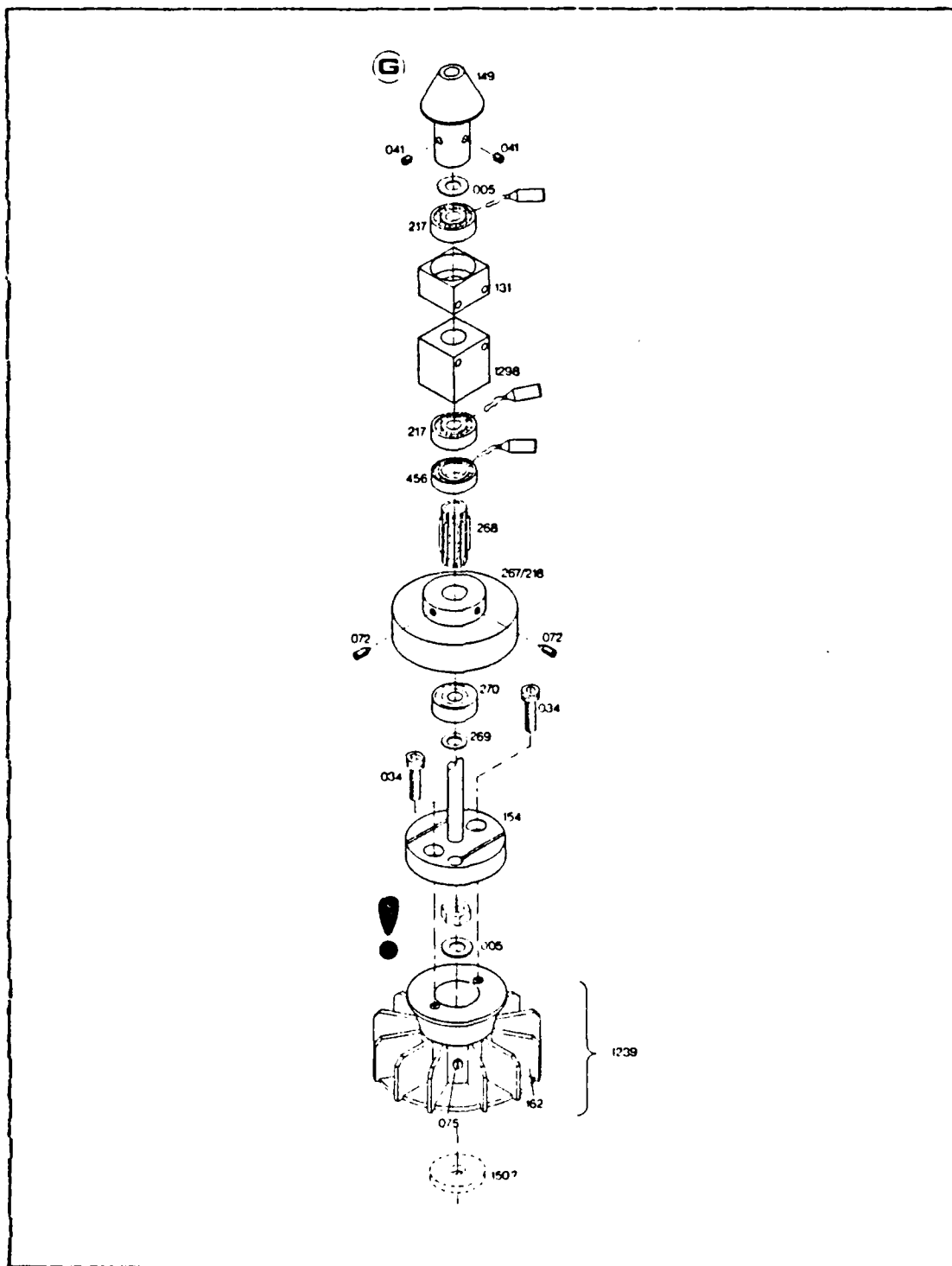
Figure A.6 Clutch Bell & Starter Cone Assembly
