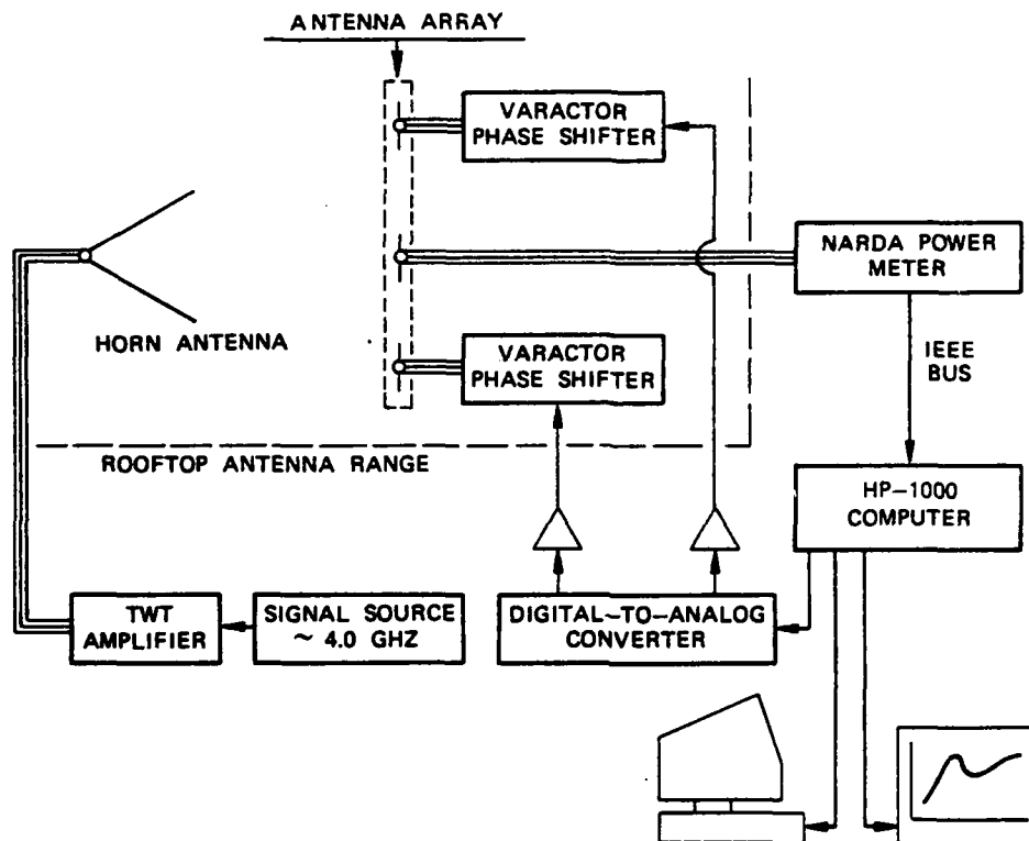
FIGURE 5. Test Setup.
