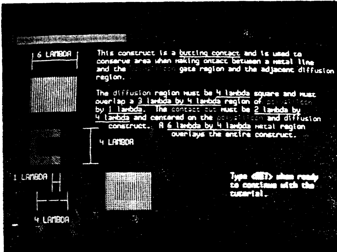
Figure B.3 Butting Contact
