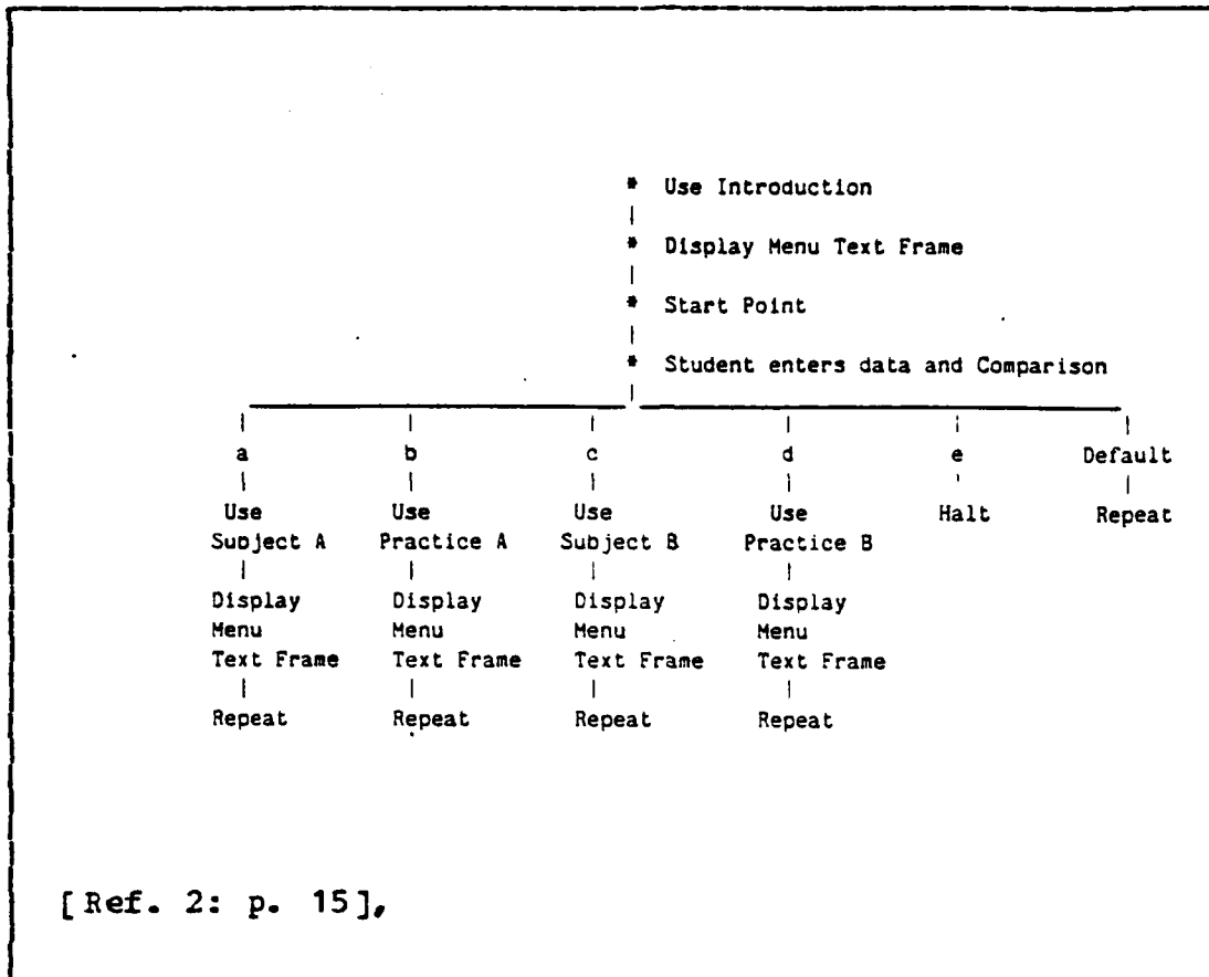
Figure 3.6 Menu Segment
