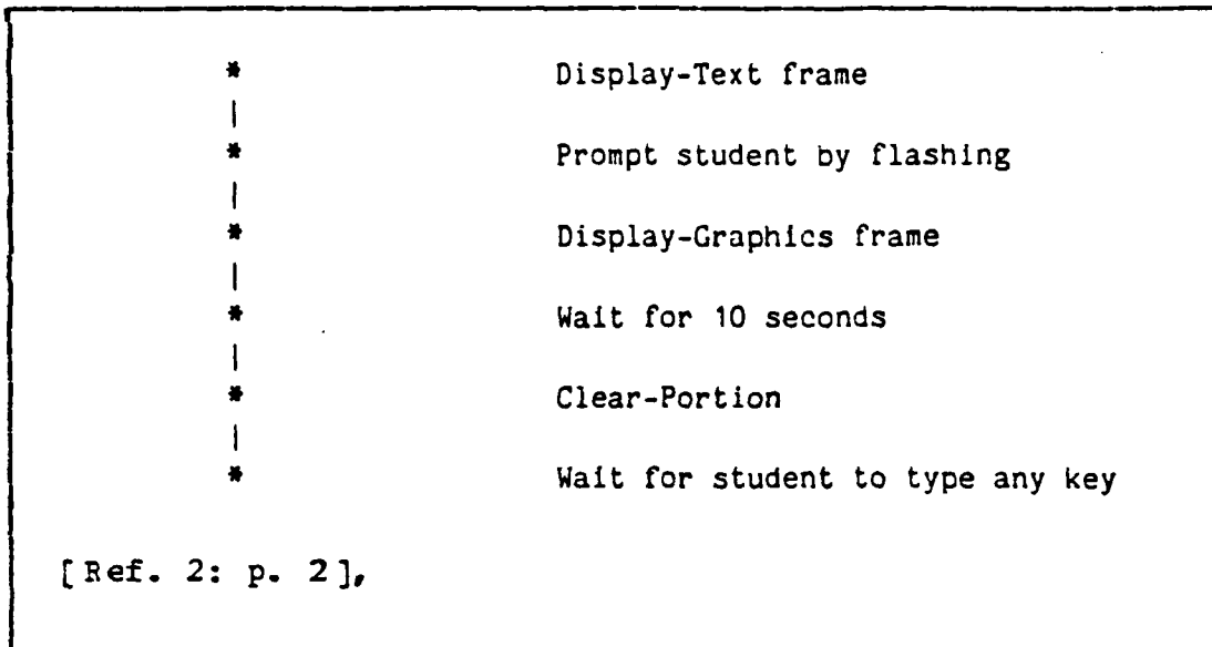
Figure 3.7 Called Segment
