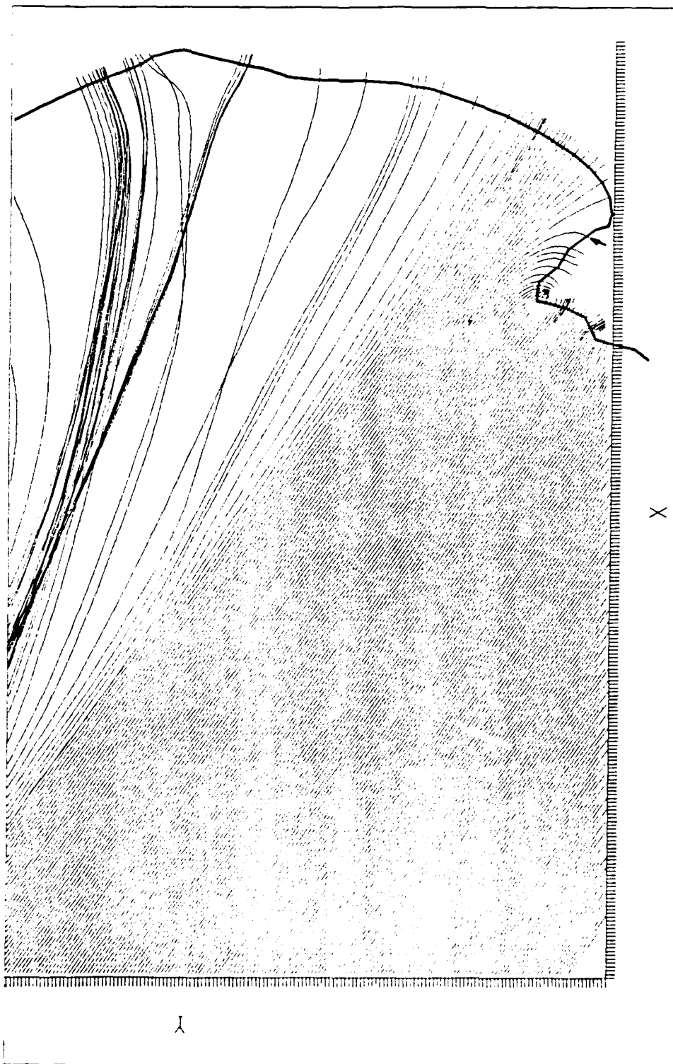
Figure 4.1 Wave Refract m (Direction: WNW , Period: 15 s)
