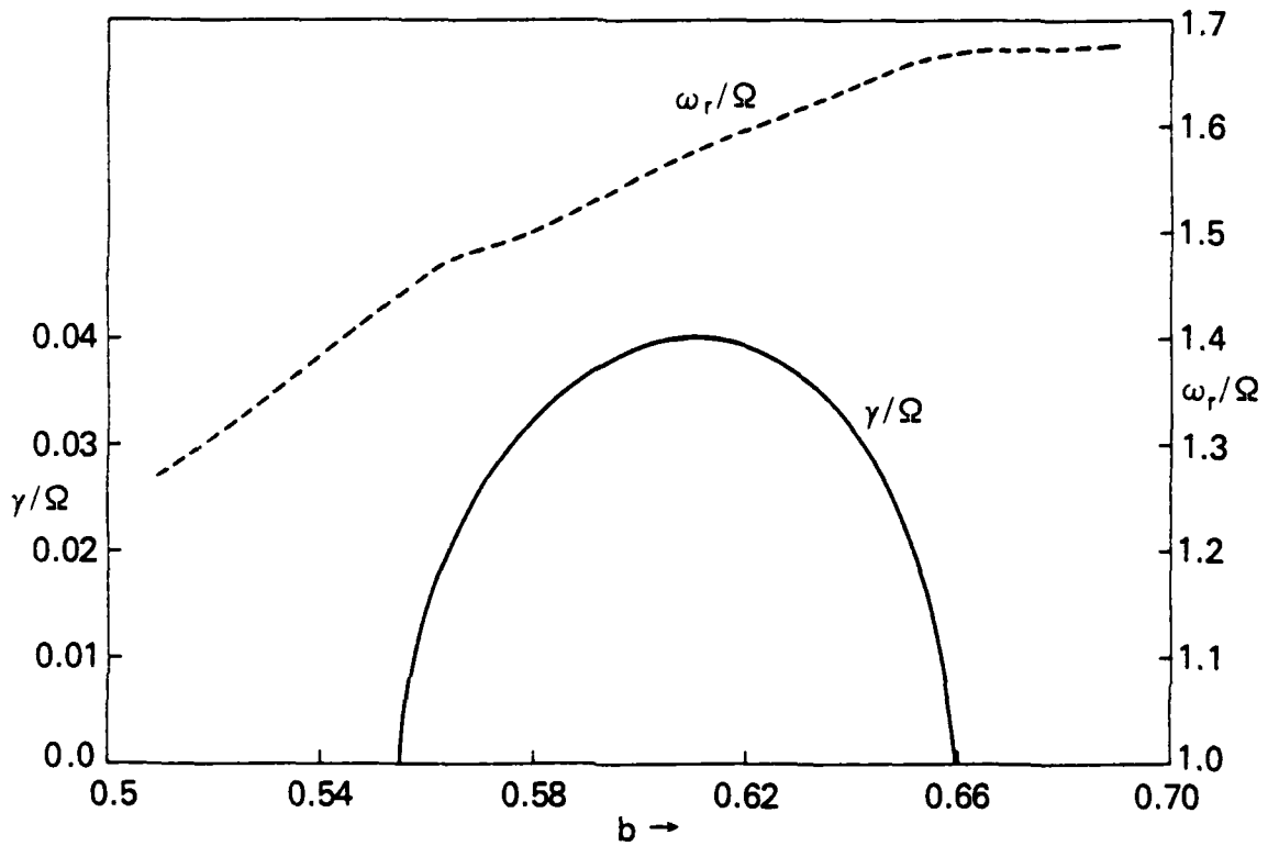
Figure 2. A plot of the real and imaginary part of the wave frequency \omega_r/\Omega_i and \gamma/\Omega_i against b . Here \tau = 0 , \nabla_E = 2.9 , \epsilon = 0.3 , \mu \approx m_i/m_e = 1837 and u = 10^{-3} .
