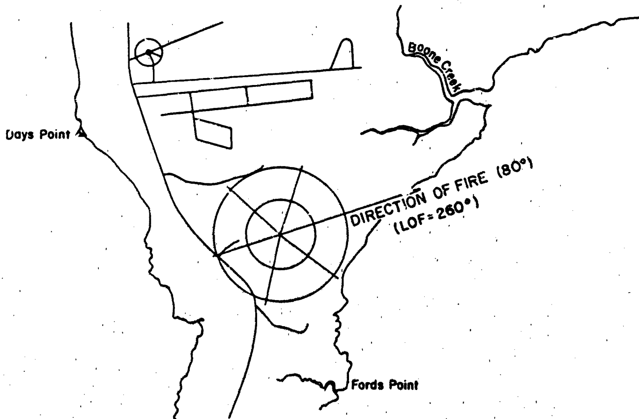
Figure 1. General site layout for noise measurements of the Bradley Fighting Vehicle 25-mm M242 main gun, Edgewood Area, APG, MD, July 1984.
