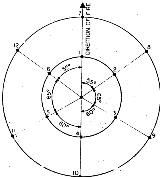
RADIUS OF INNER CIRCLE IS 750 ft, RADIUS OF OUTER CIRCLE IS 1500 ft, EXCEPT #8 IS AT 1455 ft AND #12 IS AT 1465 ft
