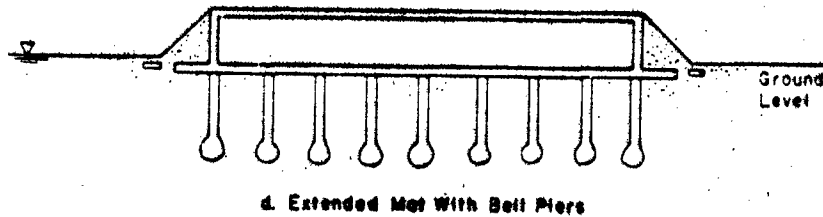
Figure 6. Aboveground configurations.
