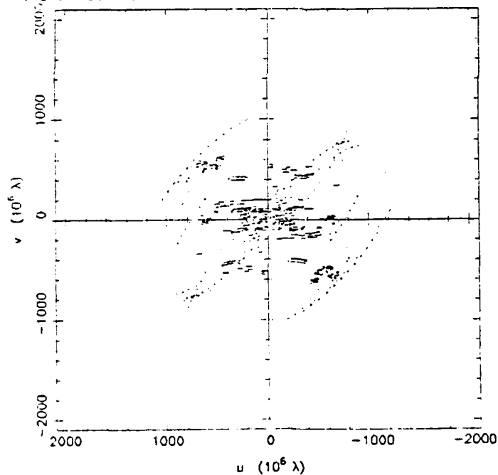
Figure 3. Same as Figure 1, except that this figure shows examples of "poor" UV-plane coverage.
