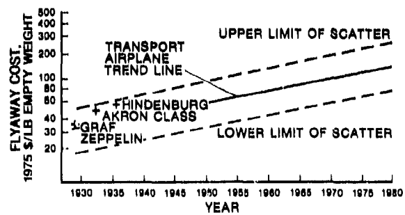
Fig. 1.6 Historical trend of flyaway costs
