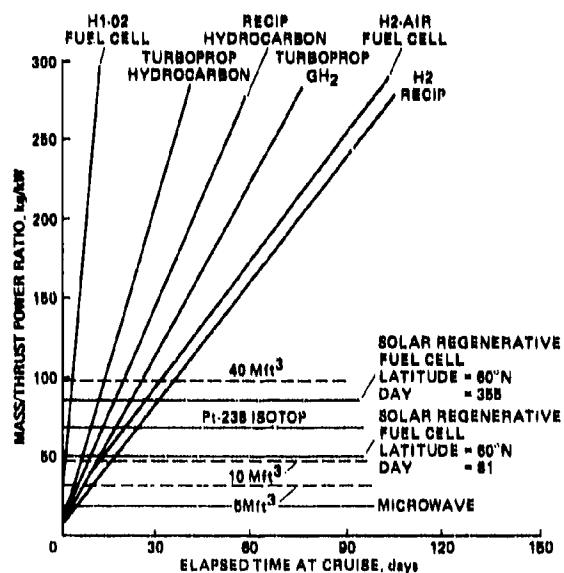
Fig. 4.3 Powertrain alternatives
