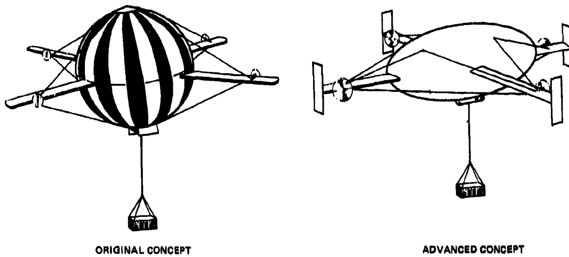
Fig. 3.7 Rotor-balloon (Aerocrane) concept
