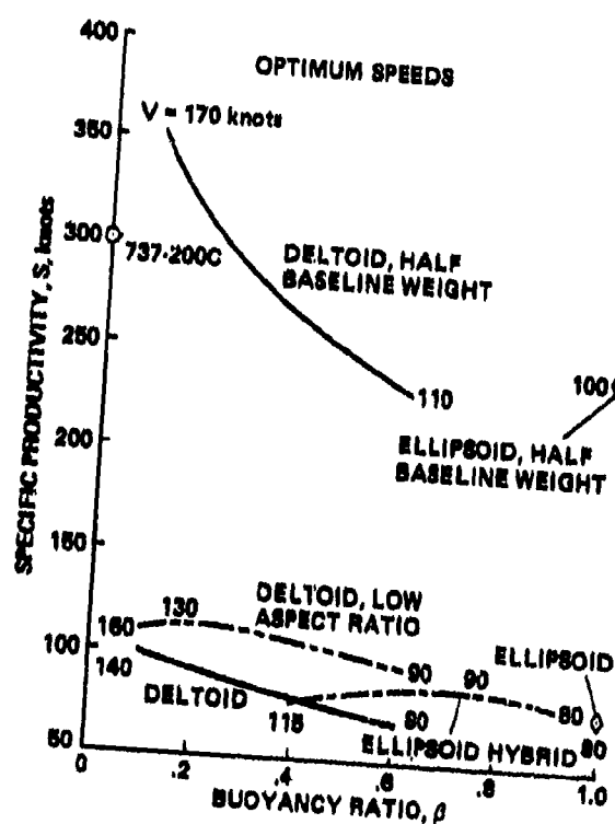
Fig. 5.5 Airship specific productivity, short-range mission
