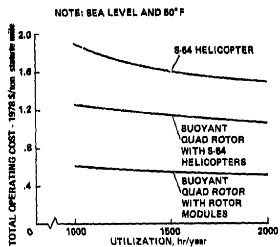
Fig. 3.6 Relative heavy-lift operating costs
