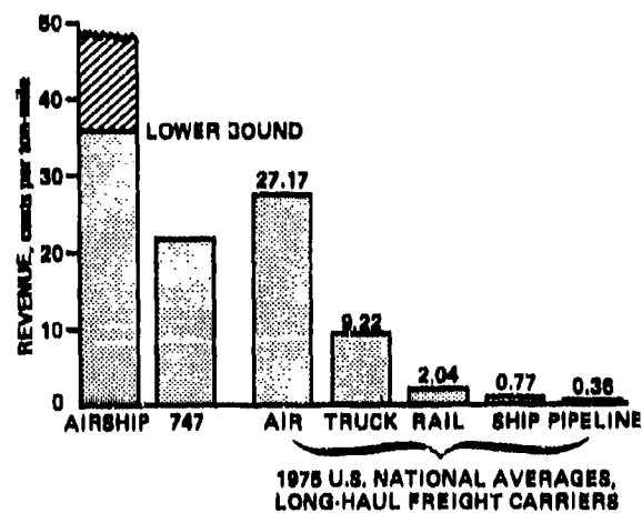
Fig. 5.8 Comparison of airship revenue with other modes
