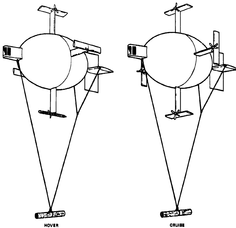
Fig. 3.9 Cyclo-Crane concept
