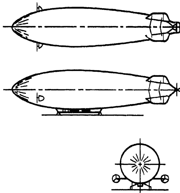
Fig. 2.3 Goodyear Aerospace patrol airship design
