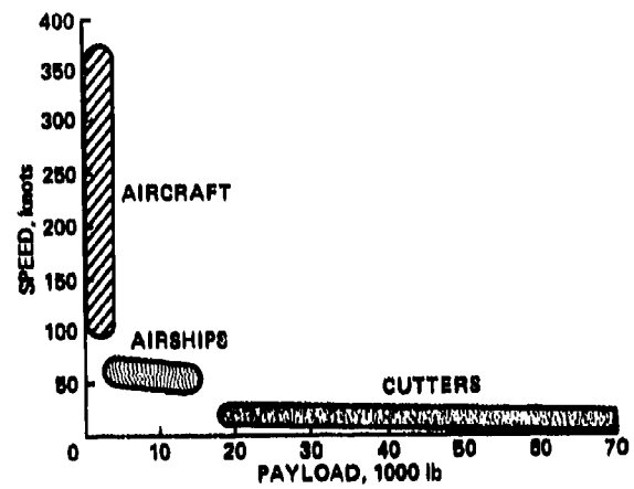
Fig. 2.2 Vehicle speed and payload
