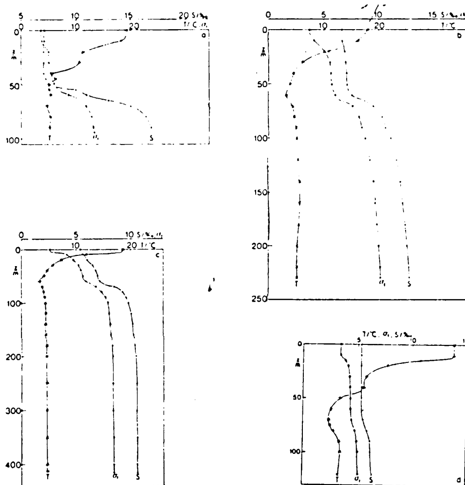
Fig. 3.2. Salinity ( S/\text{‰} ), temperature ( T/^\circ\text{C} ) and density ( \sigma_t ) profiles from: (a) Bornholm Deep 55^\circ 19.5' \text{N} , 15^\circ 38.5' \text{E} , 4.8.1938; (b) Gotland Deep 57^\circ 21.5' \text{N} , 20^\circ 02.5' \text{E} , 27.7.1938; (c) Landsort Deep 58^\circ 38.5' \text{N} , 18^\circ 16.5' \text{E} , 28.7.1938, (d) Bothnian Sea 61^\circ 04' \text{N} , 19^\circ 35' \text{E} , 12.7.1938.
