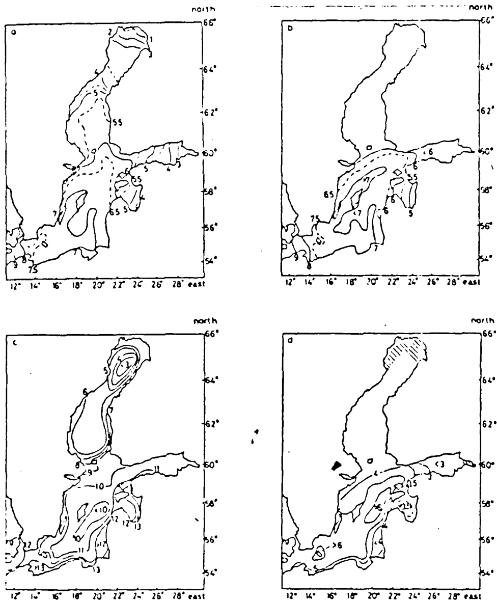
Fig. 3.1. Surface salinity ( S/^\circ\infty ) distribution for June (a) and December (b). From Bock, 1971.
