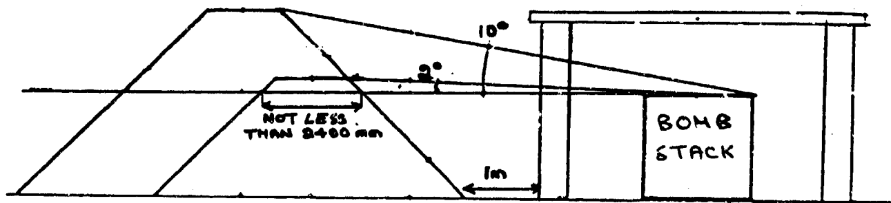
TRAVERSE DESIGN
