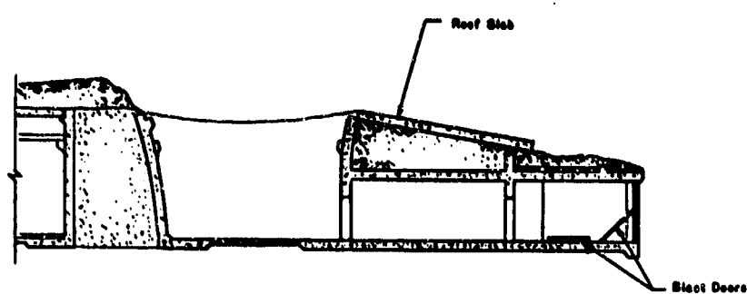
c. POST-DETONATION
