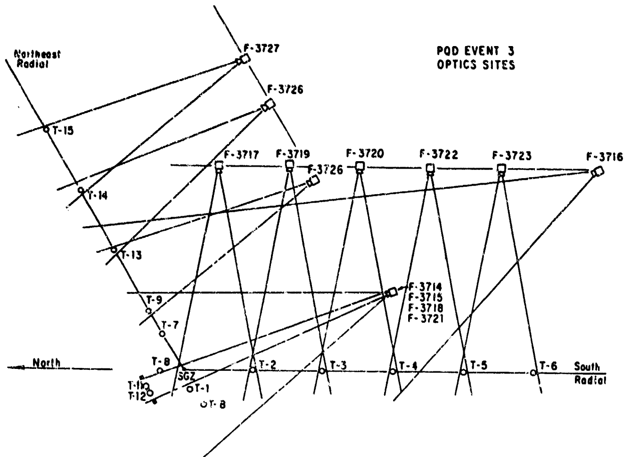
Figure 9. Camera Locations and Coverages for Debris/Ejecta Photography
