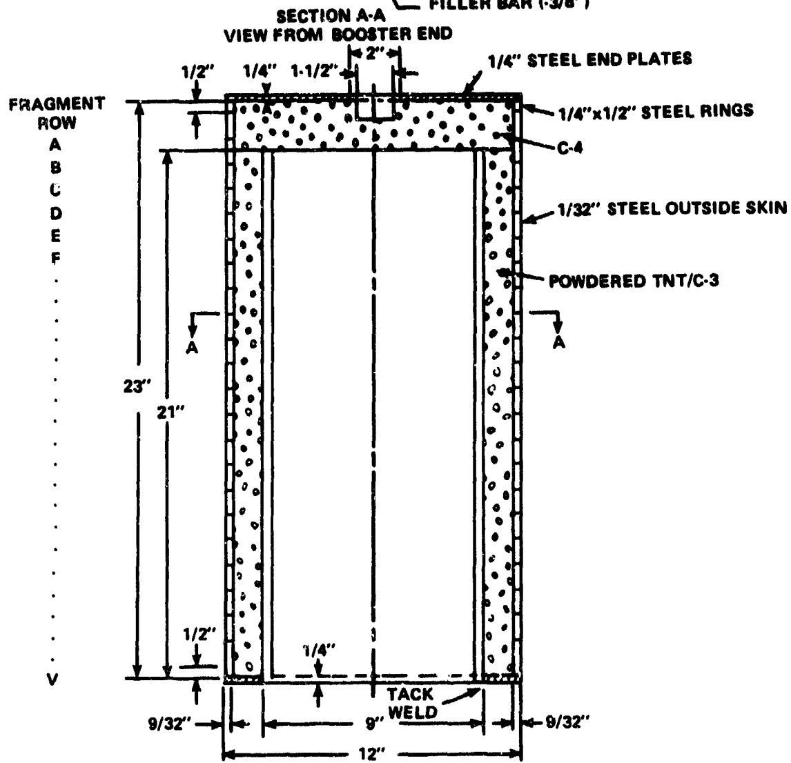
SECTION B-B FIGURE 2 WARHEAD DESIGN
