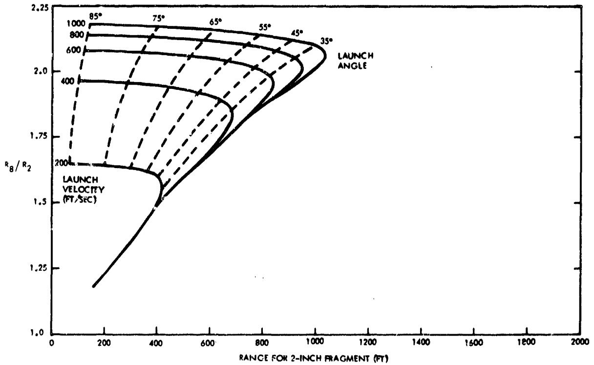
Figure 4. Comparison of Maximum Range Ratios Corresponding to QDT-3 Fragment Shape Factors and Drag Coefficient of 0.5
