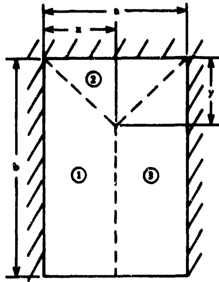
Figure 3a. Typical yield line pattern of a steel door simply supported along three sides and free along the fourth.
