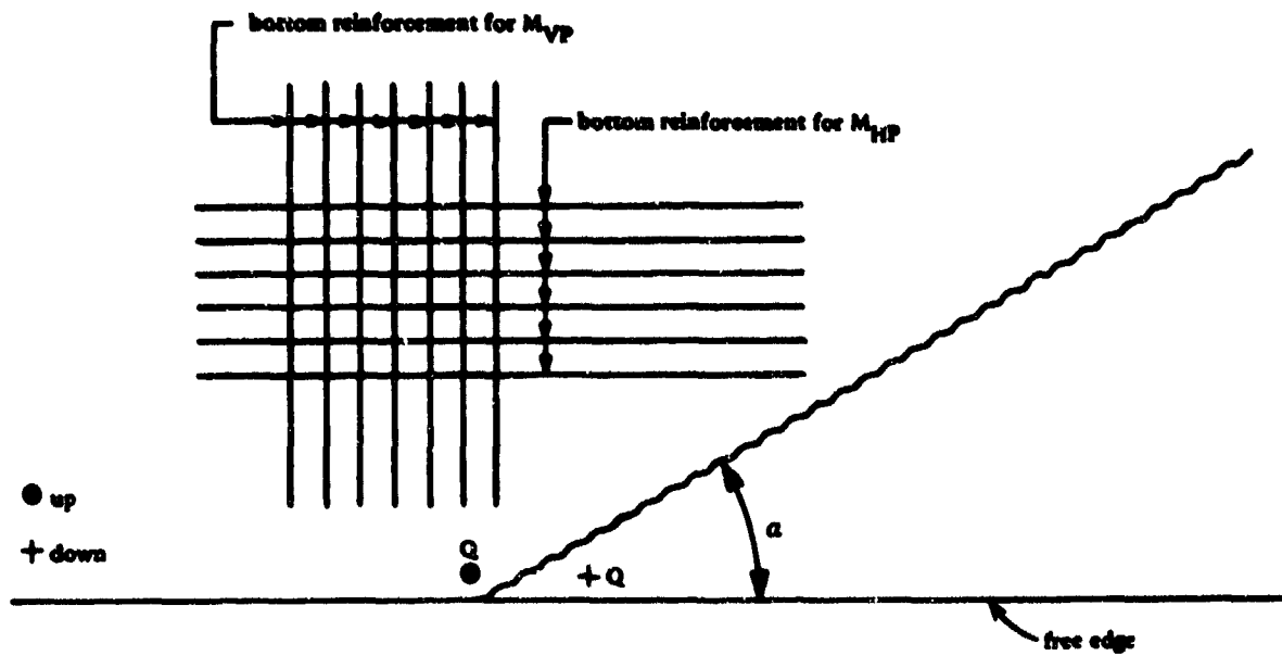
Figure 2. Nodal forces on slab with free edge.
