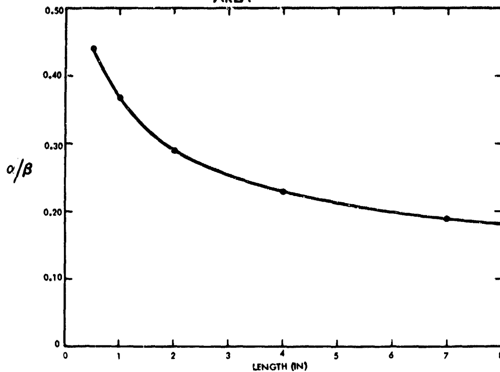
Figure 10. QDT-3 Fragment Shape Factor Variation with Length
