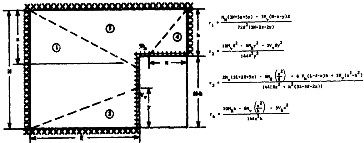
Figure 6. Yield-Line pattern #3.
