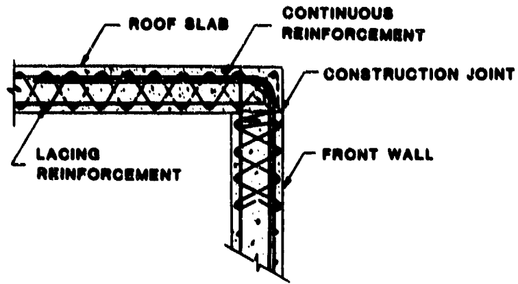
a. PRE-DETONATION
