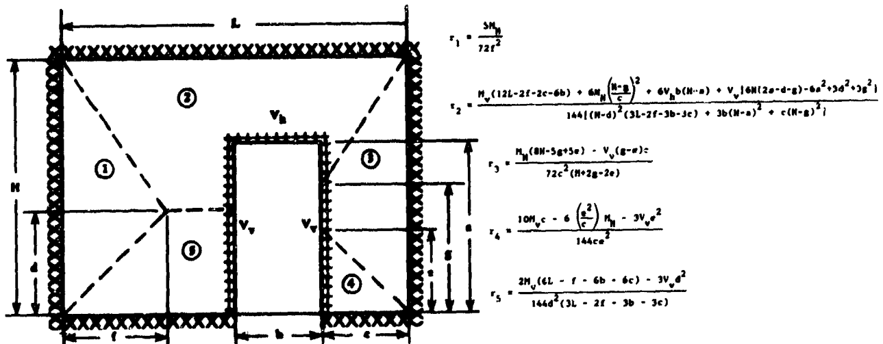
Figure 7. Yield-Line pattern #4.
