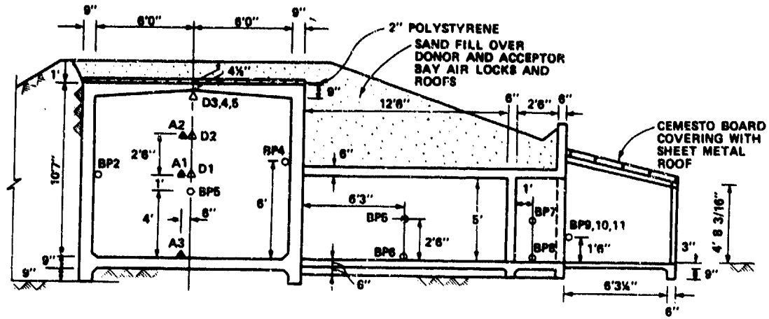
Figure 7. Elevation view of Phase II acceptor bay
