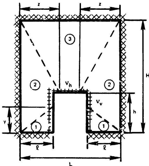
Figure 15. Yield-Line pattern #12.
