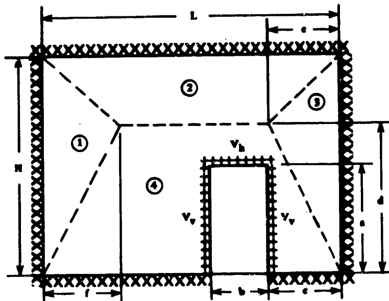
Figure 9. Yield-Line pattern #6.
