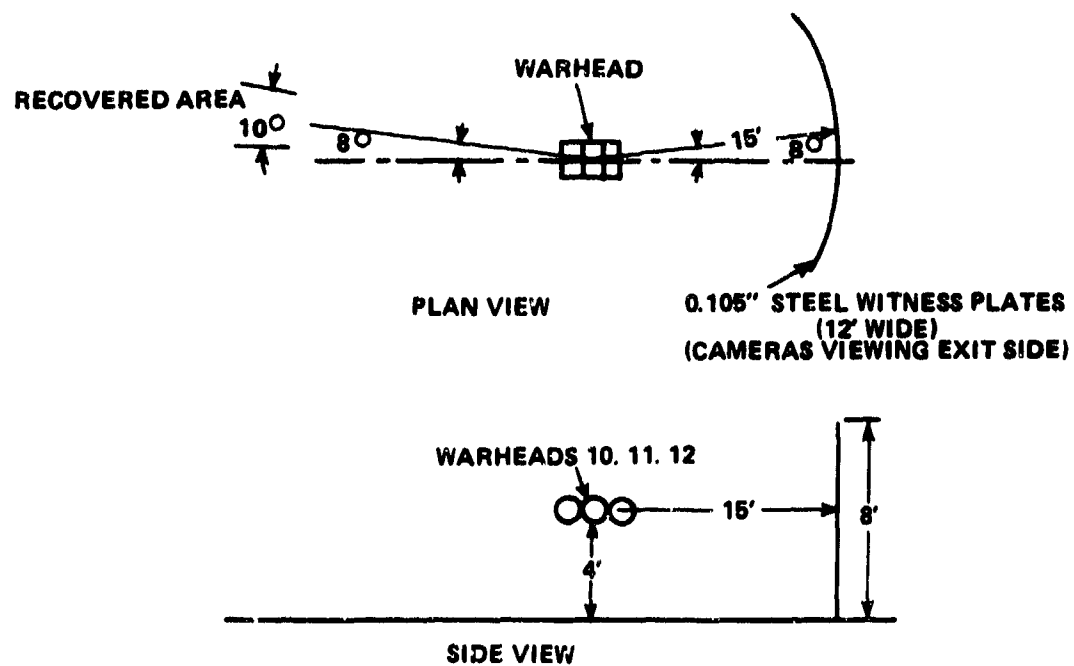
FIGURE 3B TEST ARENA FOR FRAGMENT RECOVERY TEST FOR MULTIPLE WARHEAD TEST
