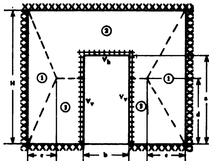
Figure 13. Yield-Line pattern #10.
