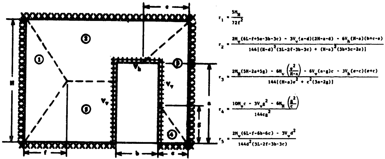
Figure 10. Yield-Line pattern #7.
