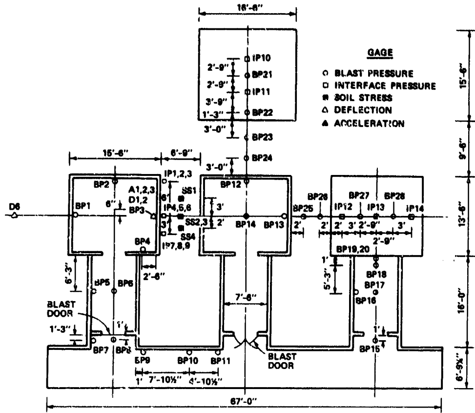
Figure 5. Plan view of Phase II structures
