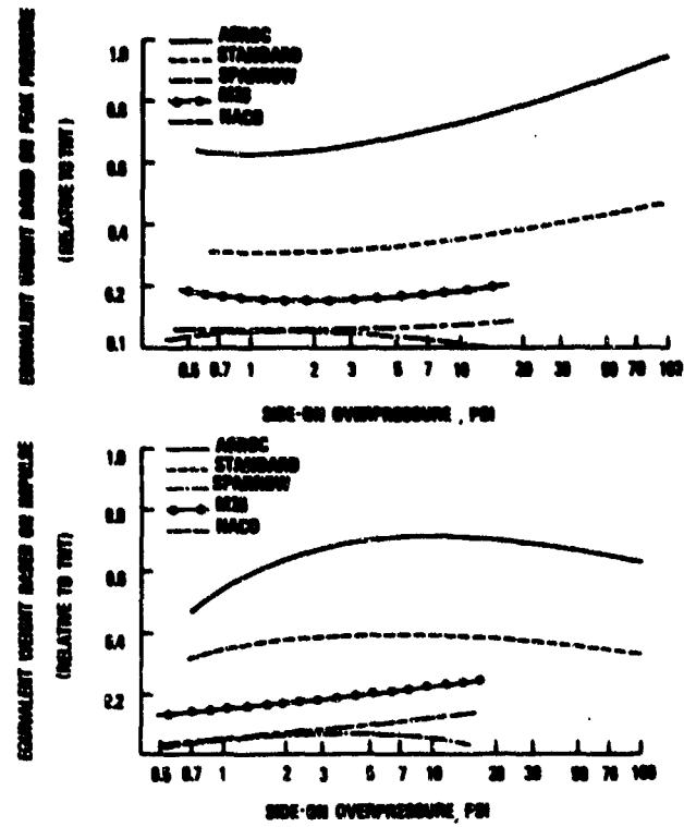
FIGURE 3 PHASE I EQUIVALENT WEIGHT VS. PRESSURE
