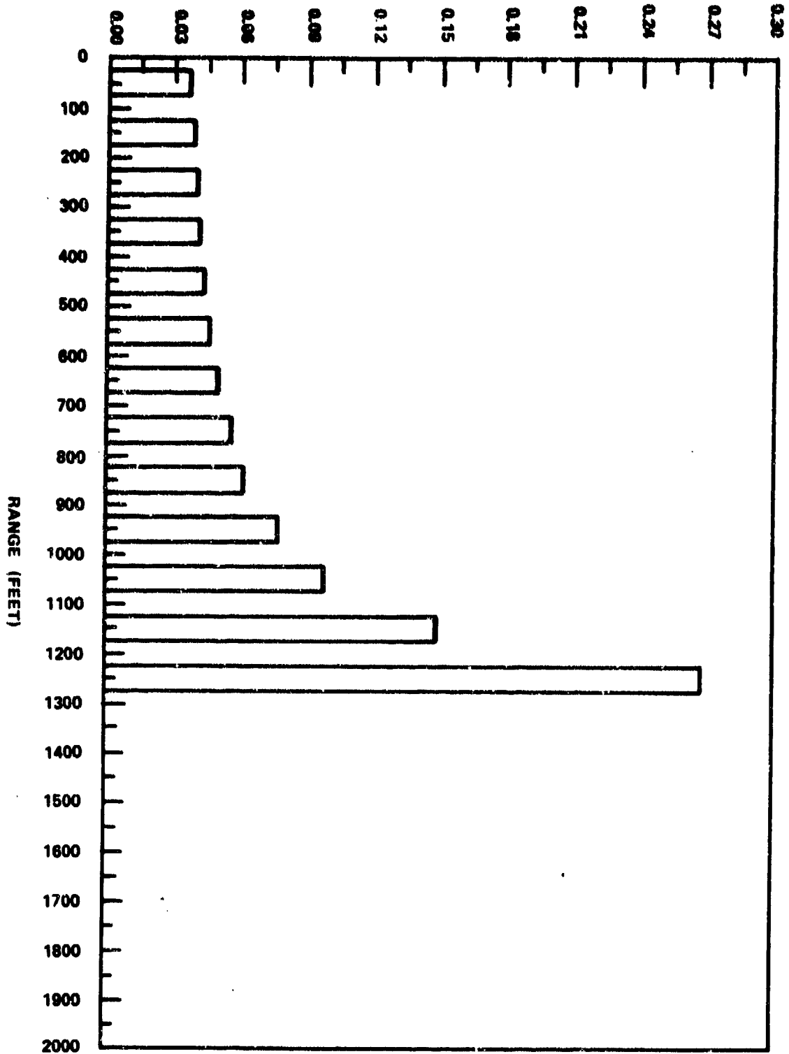
FIGURE 5A PREDICTED FRAGMENT DENSITY DISTRIBUTION
