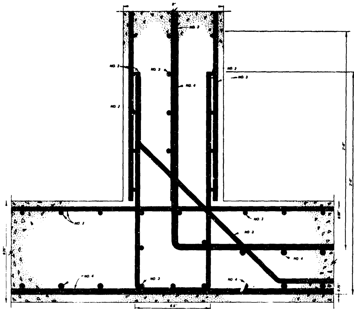
Figure 4. Elevation view, typical intersecting floor slab and wall detail (Sheet 6 of 6)
