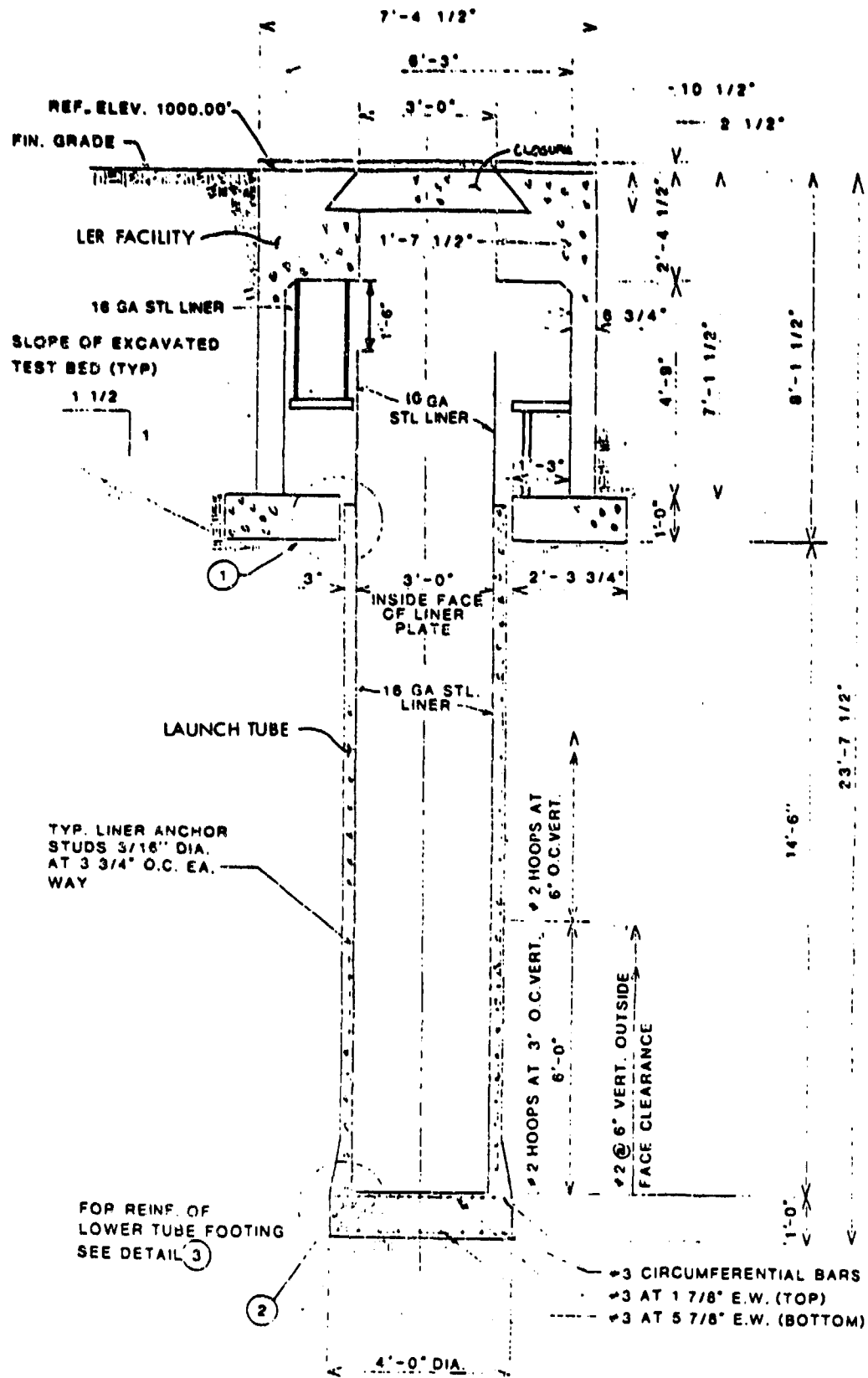
Figure 3. One-Quarter-Scale Structure
