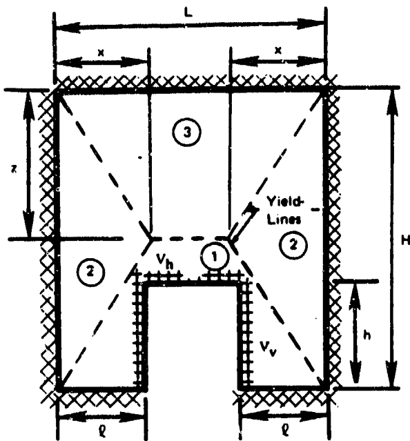
Figure 14. Yield-Line pattern #11.
