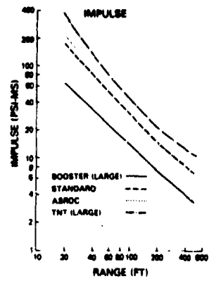
FIGURE 1 PHASE I AIRBLAST COMPARISONS
