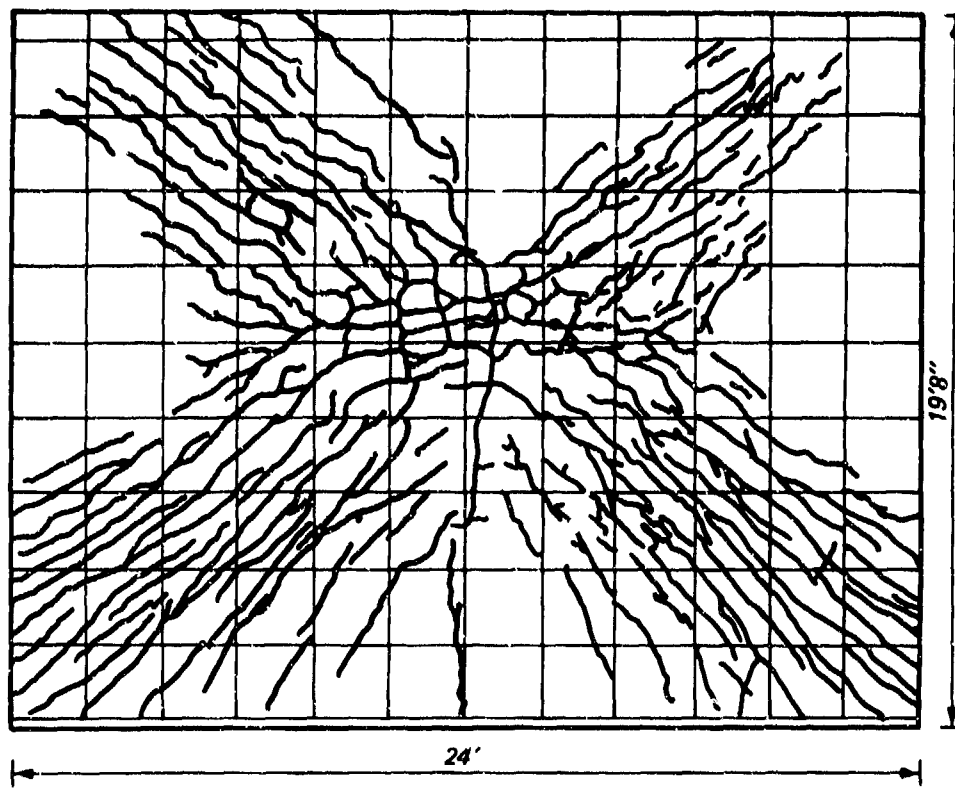
Figure 11. Posttest crack pattern on Phase I acceptor bay wall
