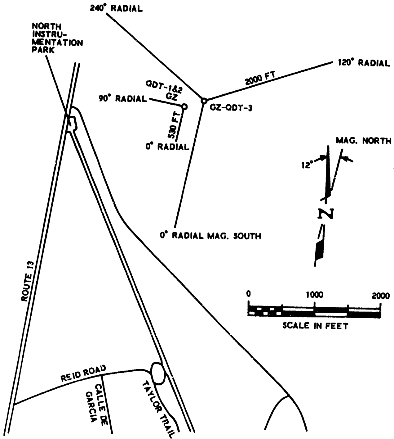
Figure 6. Test Site Layout for QDT-1, QDT-2, and QDT-3
