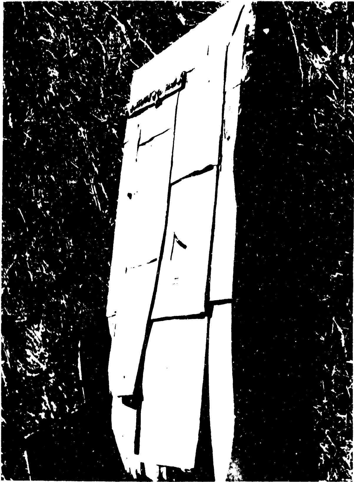
Figure 13. Test Results - Test No. 7, 7.3 Kg TNT Charge Positioned Inside Magazine 4 Metres from Headwall.
