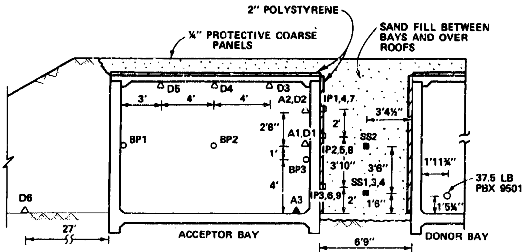
Figure 6. Elevation view of Phase II donor and acceptor bays
