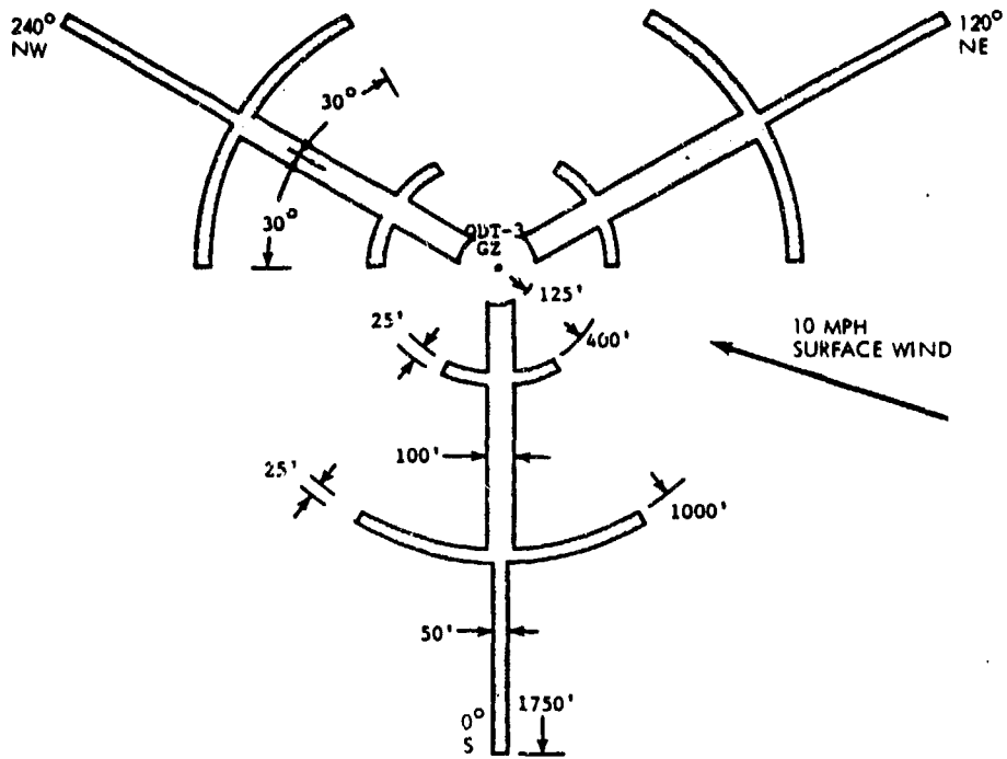
Figure 7. Locations of Areas Requiring Brush Clearing for Airblast Gages and Ejecta Surveys
