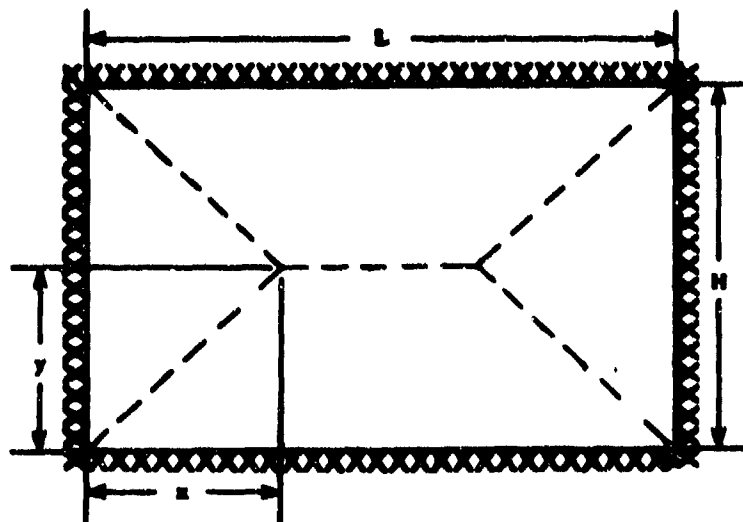
Figure 1a. Typical yield lines for a rectangular slab.
