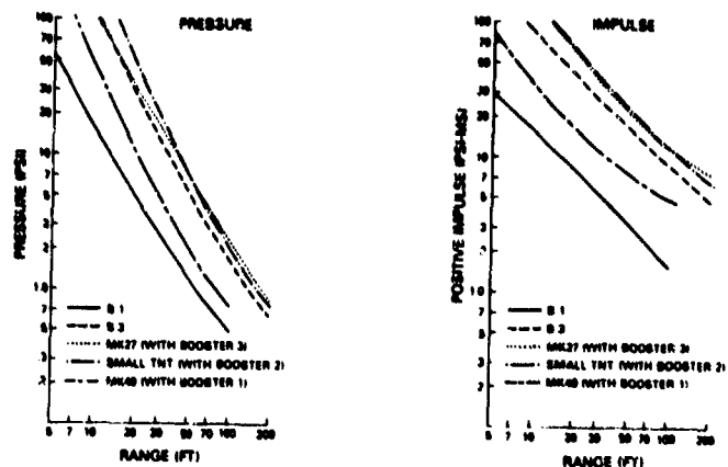
FIGURE 2 PHASE II AIRBLAST COMPARISONS
