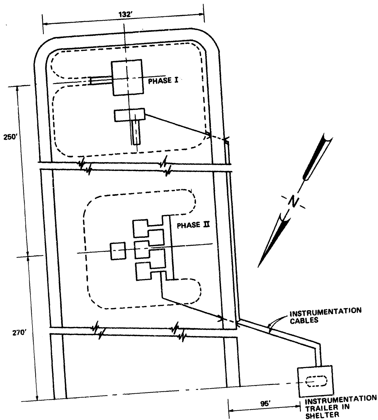
Figure 1. Test site layout at Camp Shelby, MS
