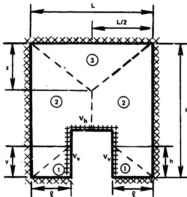
Figure 12. Yield-Line pattern #9.
