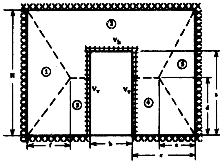
Figure 8. Yield-Line pattern #5.
