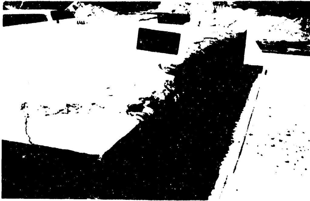
Figure 8. Outside view of damaged roof after Test 2. Note damage at edge of roof and crack in concrete at corner
