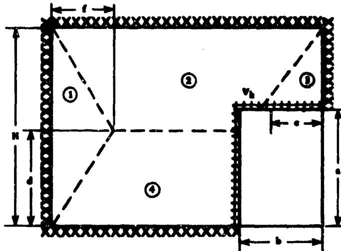
Figure 5. Yield-Line pattern #2.
