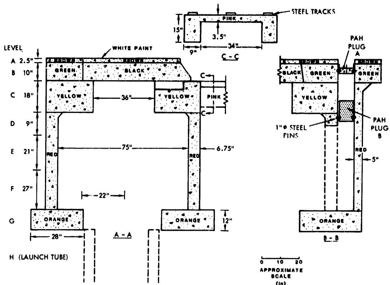
Figure 4. One-Quarter-Scale LER Cross-Sections
