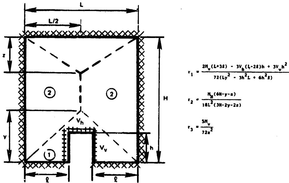
Figure 11. Yield-Line pattern #8.
