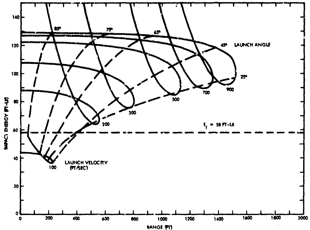
Figure 1. Fragment Size Limitation for Impact Energy Criterion (Continued)
