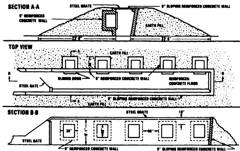
Figure 3 - Magazine Arrangement at Bethesda
