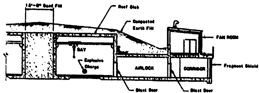
a. PRE-DETONATION
