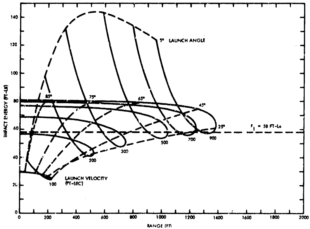
Figure 1. Fragment Size Limitation for Impact Energy Criterion
