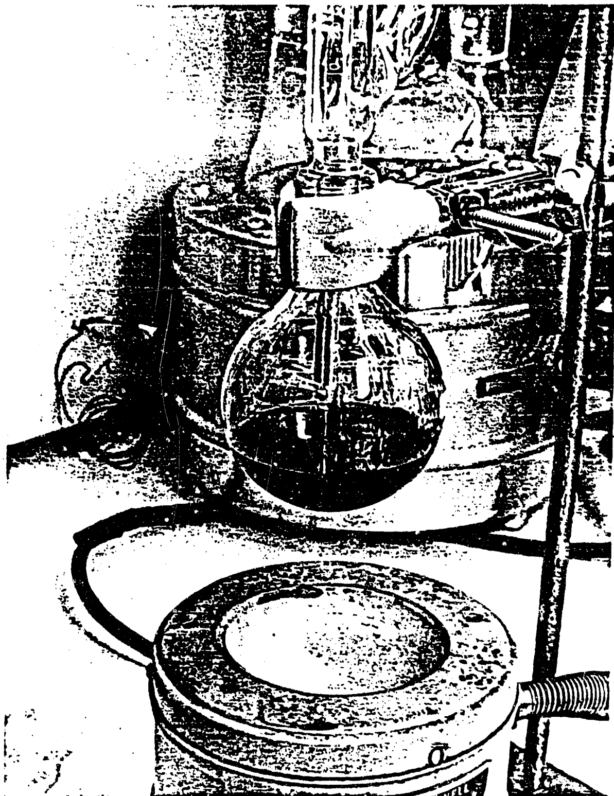
DISSOLUTION / CONVERSION SEQUENCE OF YELLOW D SLURRY IN n -BUTYLAMINE AFTER 1 HOUR AT 70° C.
