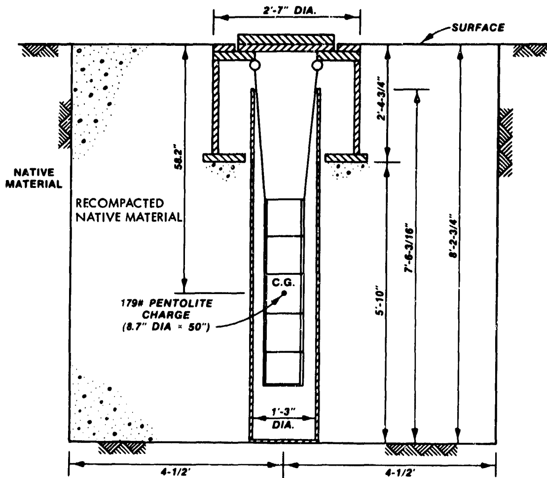
Figure 2. One-Tenth Scale Test Article and Test Bed Configuration
