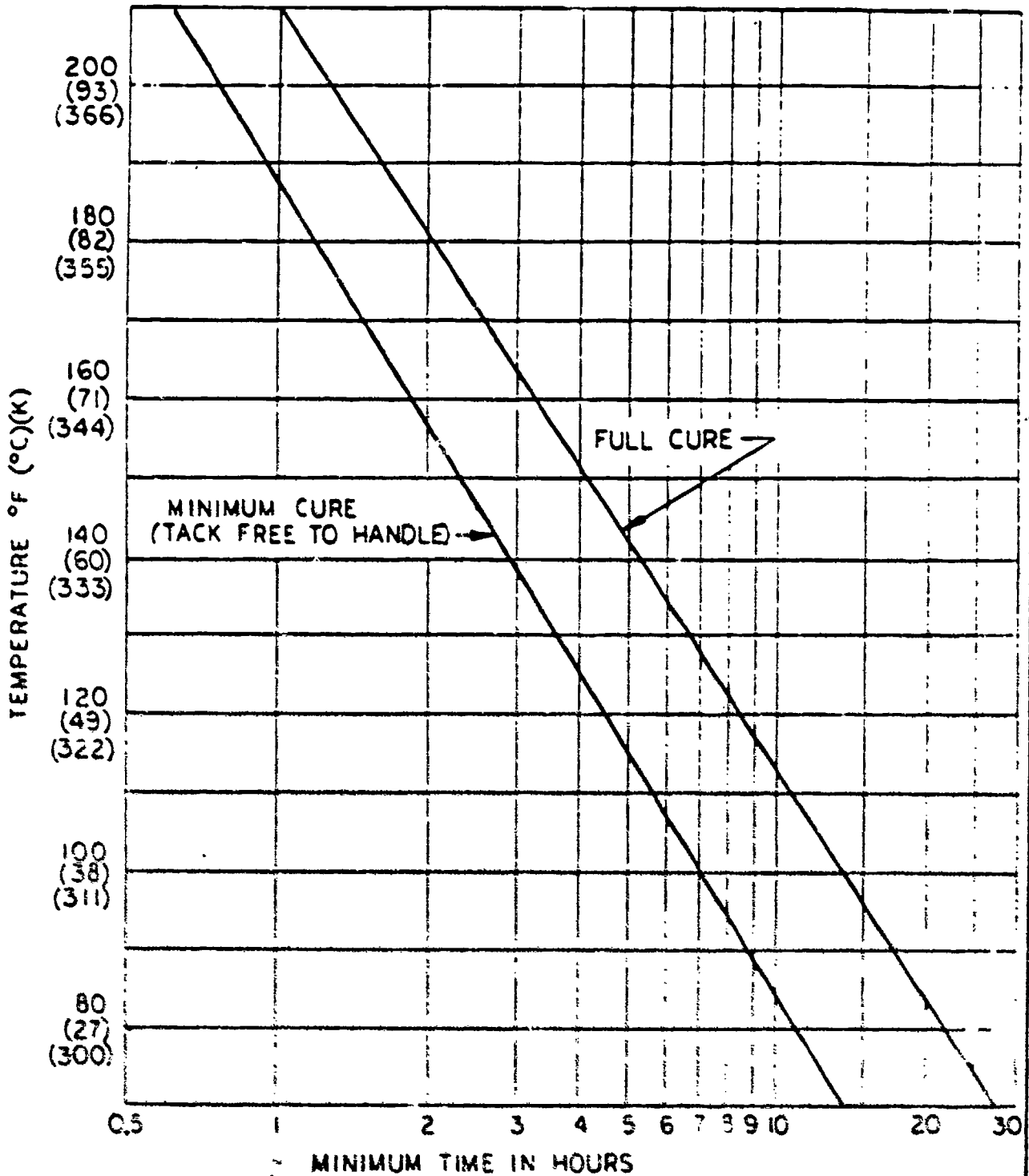
FIGURE 1. CURE CYCLE
