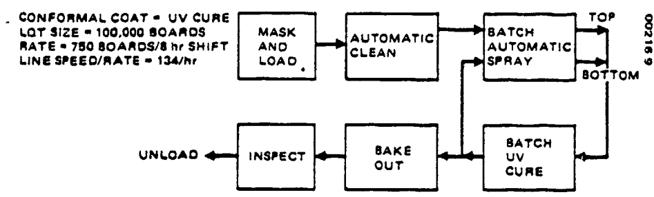
FIGURE 6. PROPOSED UV PWB COATING WORK FLOW DIAGRAM
