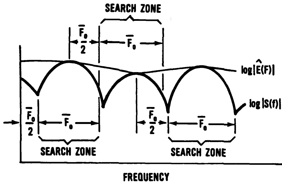
Figure A3-17. Spectral envelope estimator. (Taken from ref. 99, p. 787)
