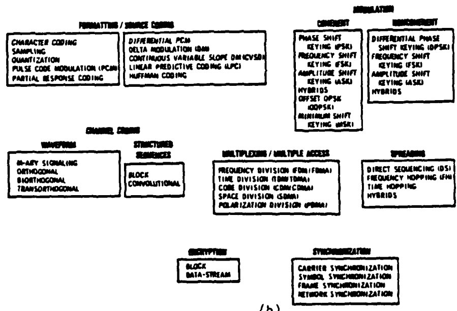
Figure 2-1. Digital communication system; (a) typical block diagram and (b) basic digital communication transformations. (Taken from ref. 54)
