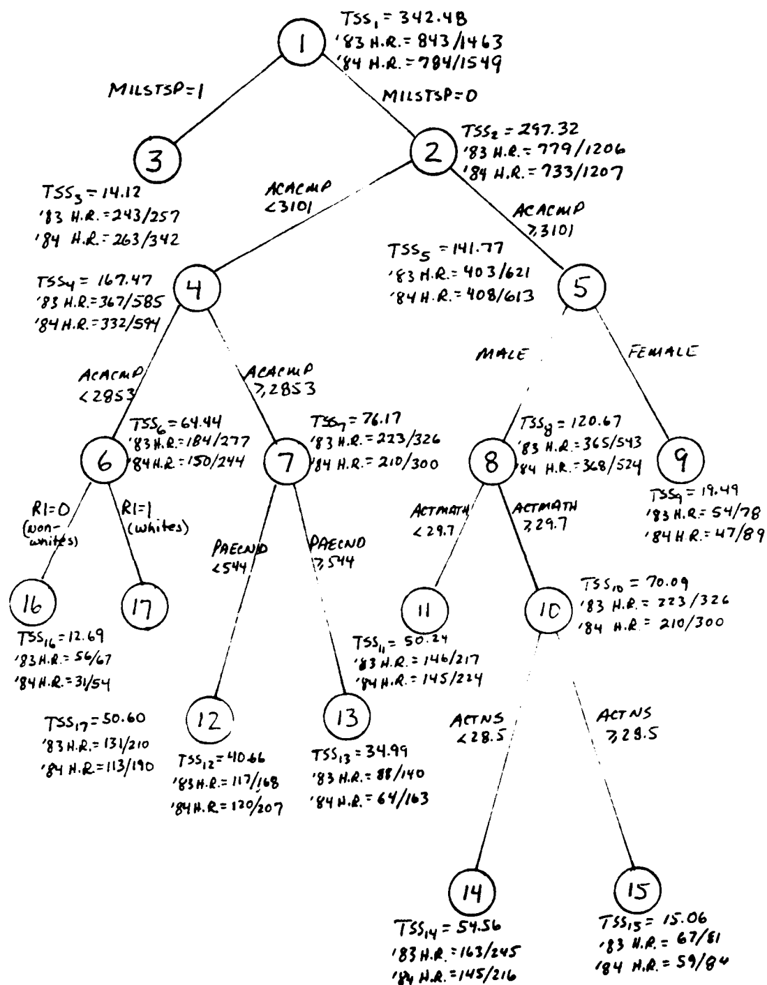
Figure 11. Tree Diagram after Eight Splits
