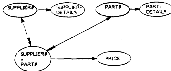
Figure 22. Concatenated Keys (10:184)
