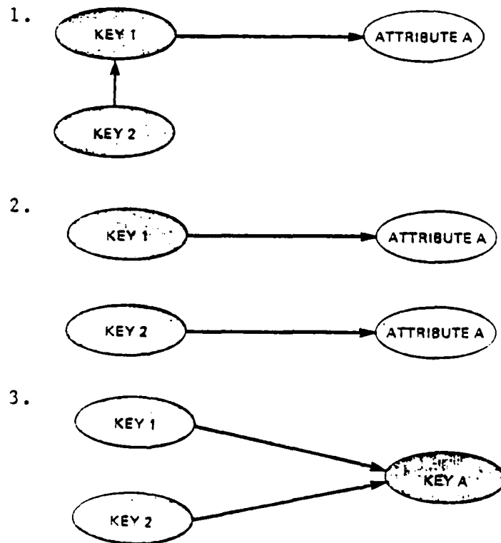
Figure 24. Intersecting Attributes (10:247-248)
