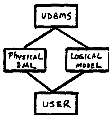
Figure 8. Bi-model Approach
