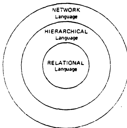
Figure 11. Onion-Layered Approach (3:451)
