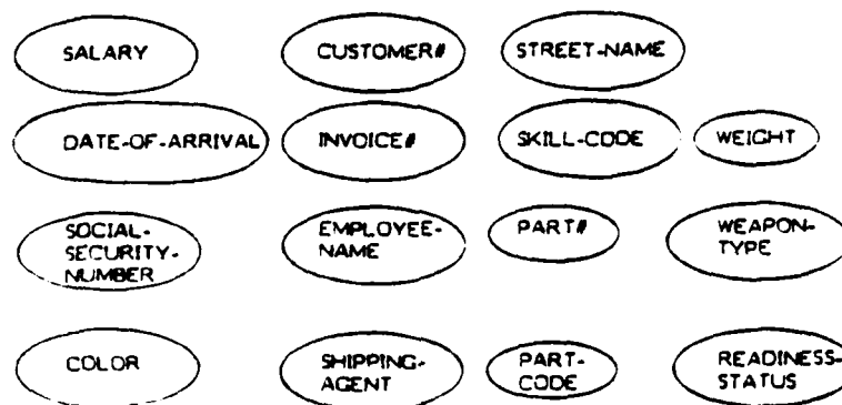
Figure 12. Canonical Bubbles (10:172)
