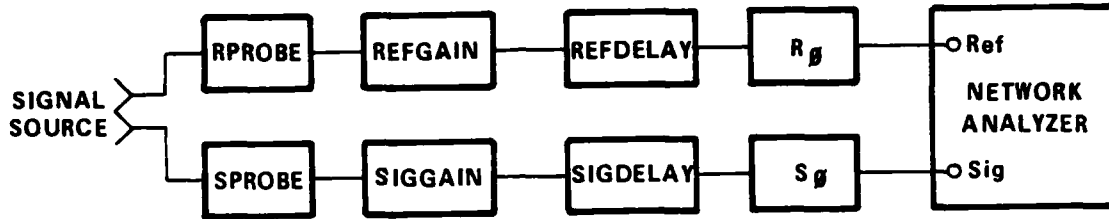
Figure 2-1. Test Network Configuration
