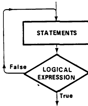
Figure 6-3. Flowchart of REPEAT construct
