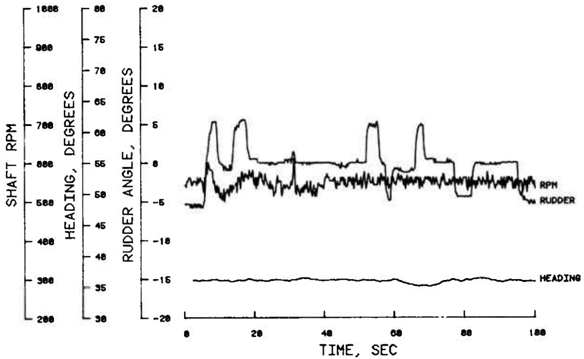
Figure 20. Model ship data--safe transit; W/B = 2.50 , H/T = 1.2
