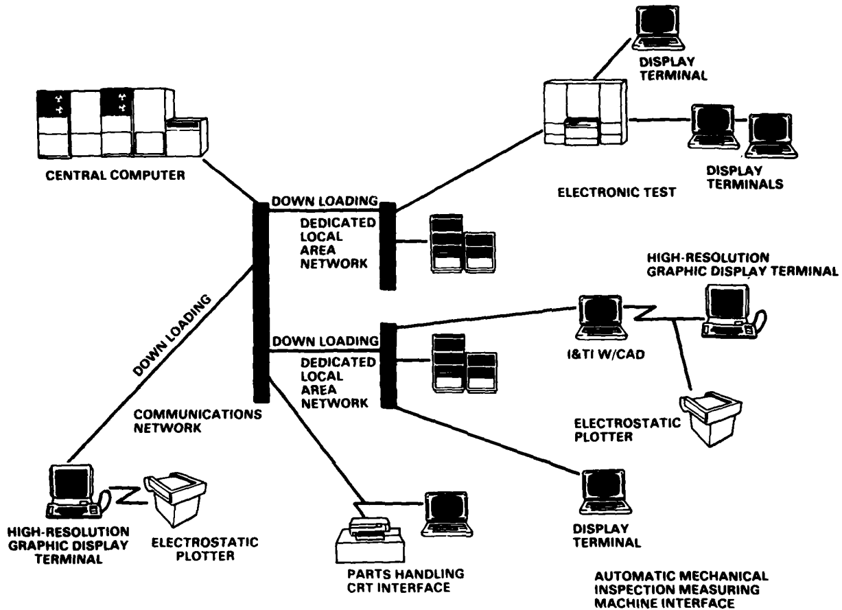
Data Network
