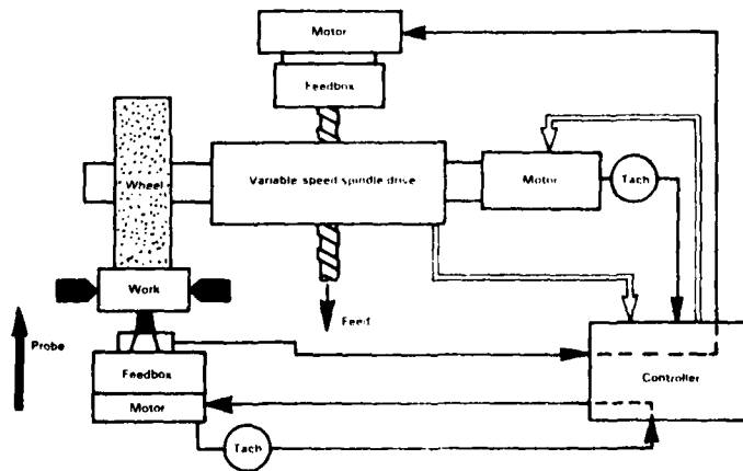
Energy-adaptive grinder
