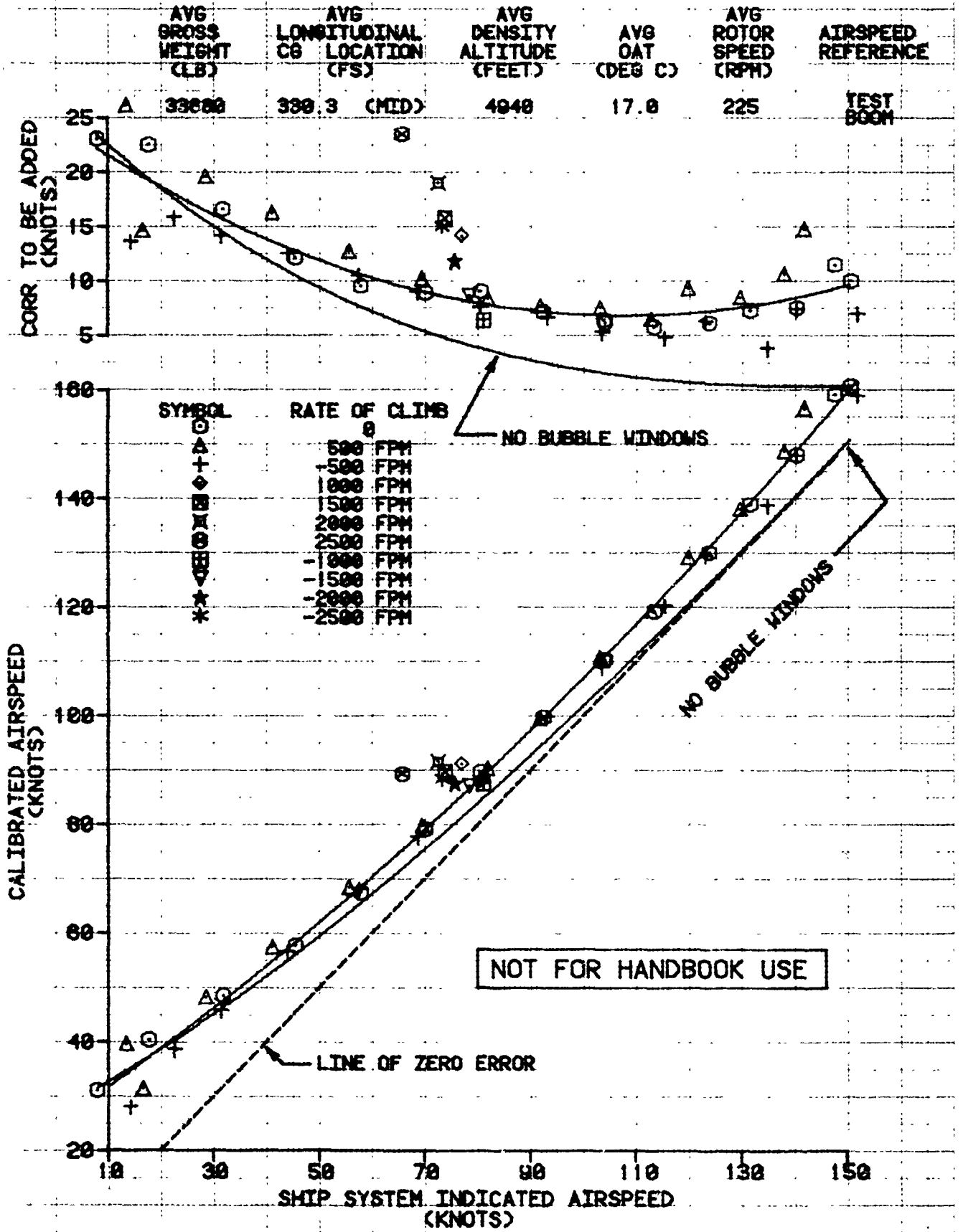
FIGURE 140 SHIPS SYSTEM AIRSPEED CALIBRATION CH-47D USA S/N 81-23383 BUBBLE WINDOWS INSTALLED
