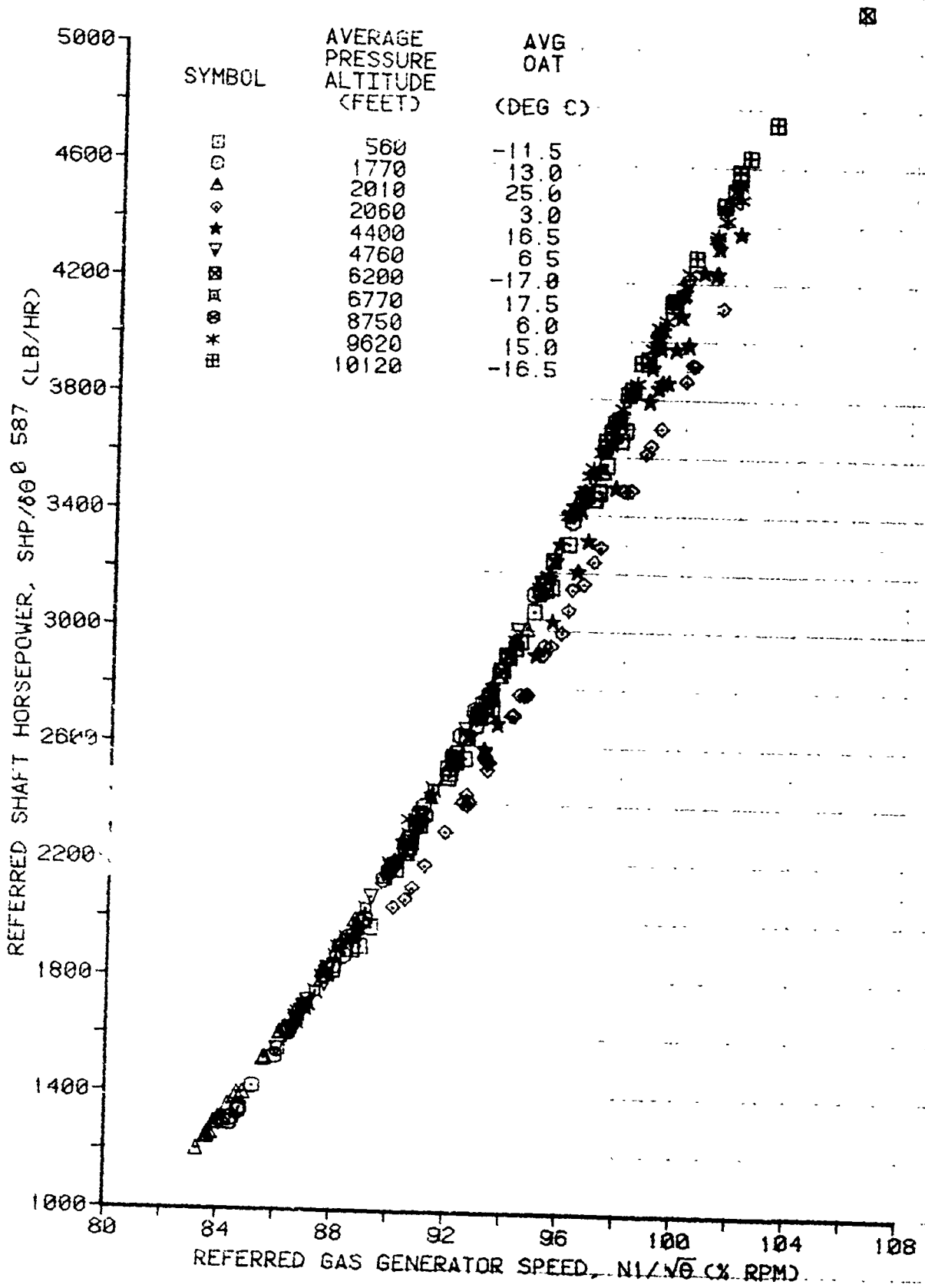
FIGURE 149 ENGINE CHARACTERISTICS CH-47D USA S/N 81-23383 LYCOMING T55-L-712 S/N 71226
