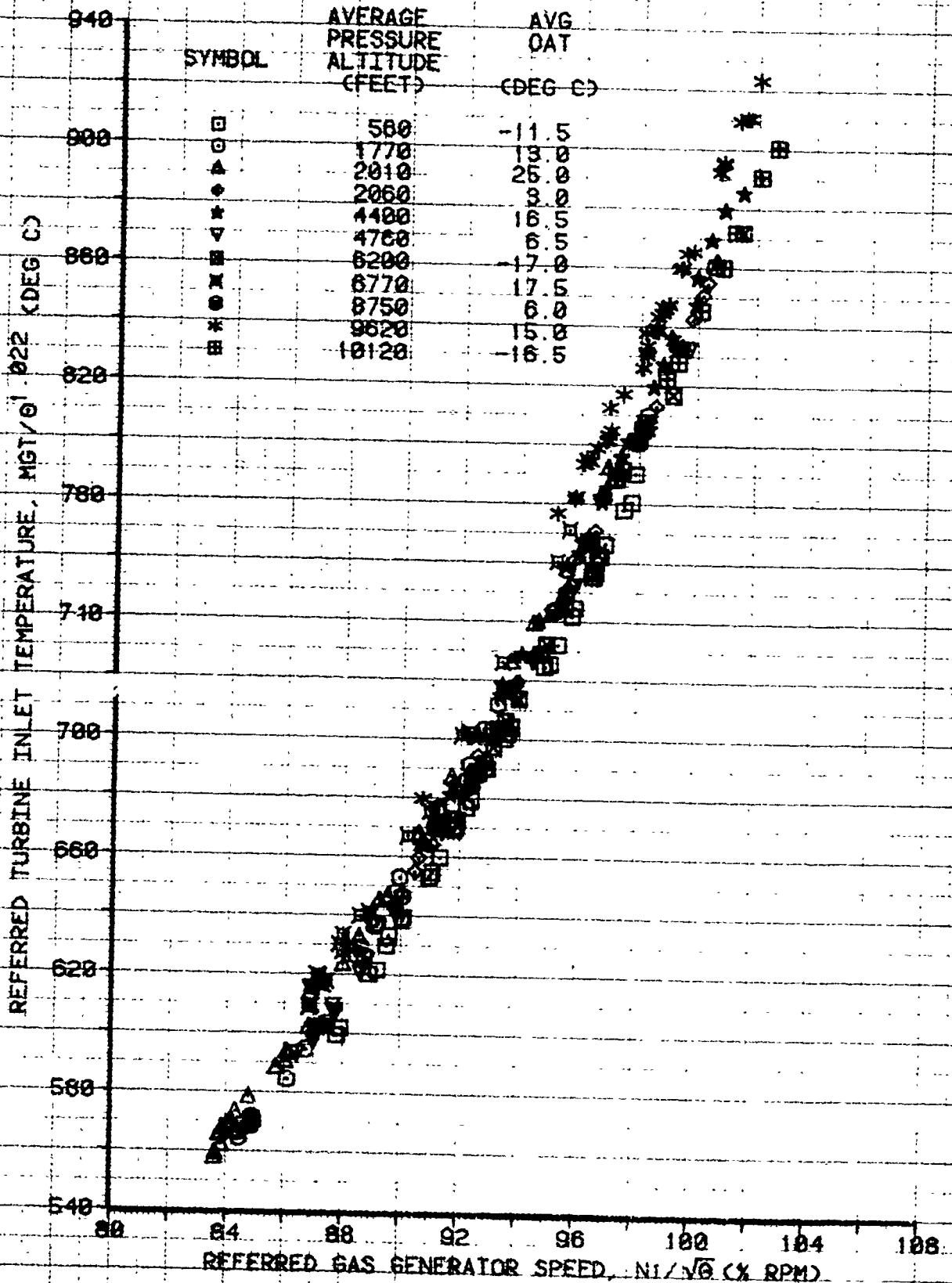
FIGURE 148 ENGINE CHARACTERISTICS CH-47D USA S/N 81-23383 LYCOMING T55-L-712 S/N 71224
