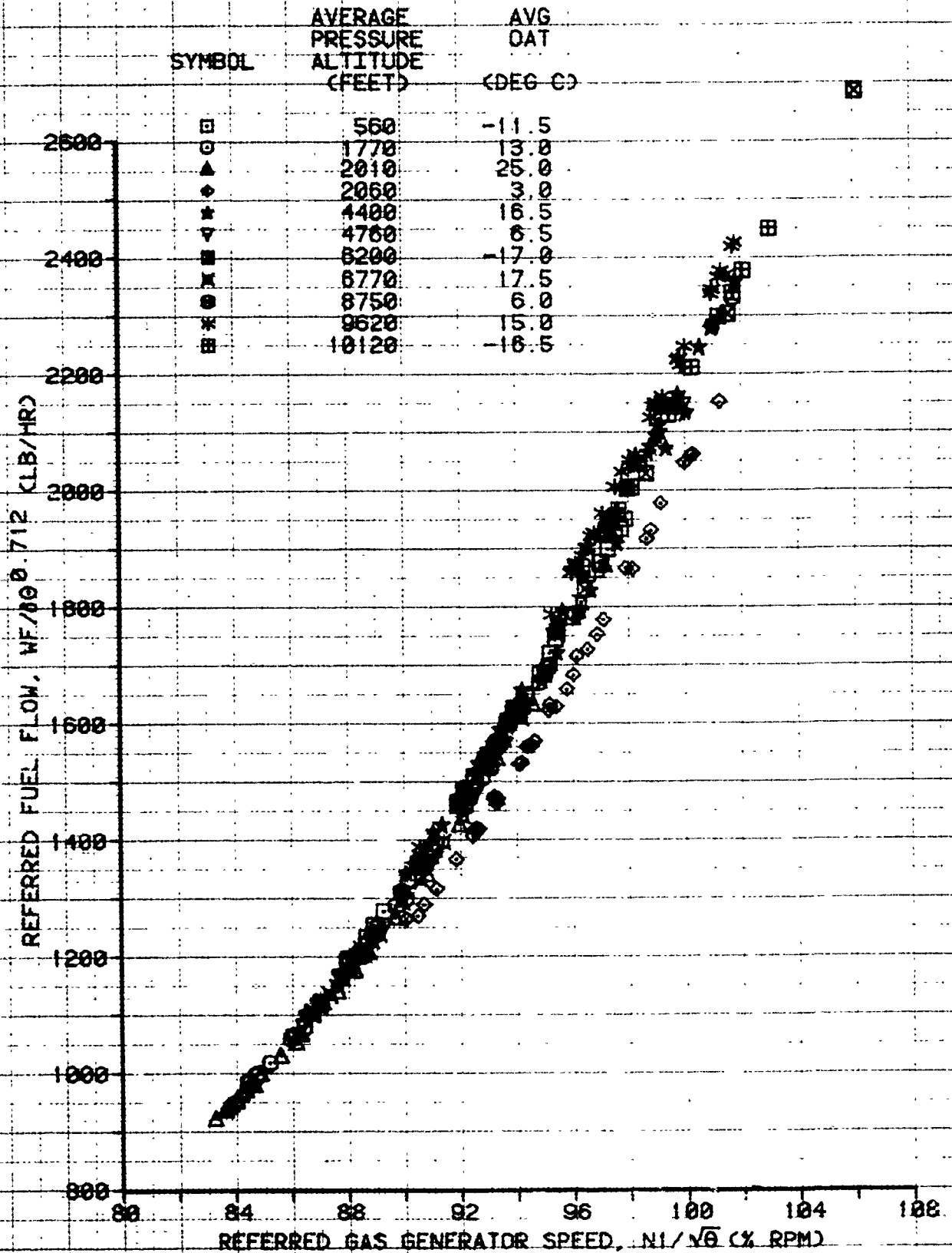
FIGURE 150 ENGINE CHARACTERISTICS CH-47D USA S/N 81-23383 LYCOMING T55-L-712 S/N 71226
