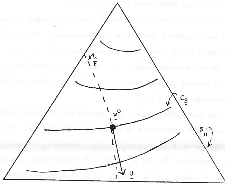
Figure 1. All probability distributions supported on \{x_1, x_2, \dots, x_n\} are represented as the simplex S_n . The central point w^0 corresponds to the empirical distribution \hat{F} . The curves indicate level surfaces of constant value of the parameter \theta . In particular C_{\hat{\theta}} comprises those probability distributions having \theta equal to \theta(w^0) = \hat{\theta} , the MLE. The least favorable family \hat{F} passes through w^0 in the direction U , orthogonal to C_{\hat{\theta}} .
