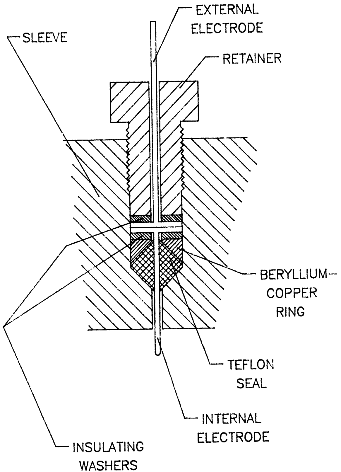
Figure 5. Firing Electrode
