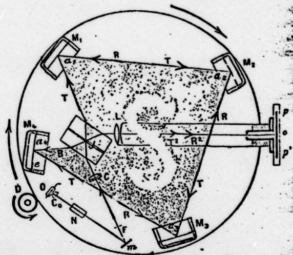
FIG. 2. Sagnac's original interferometer.
