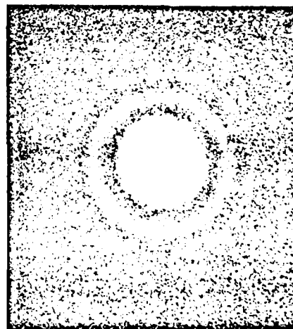
Fig. 2. The observed fringe pattern. High contrast was obtained by equalizing the spatial intensity distributions of both beams.
