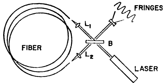
Fig. 1. Experimental configuration of the optical components: L_1 and L_2 are the converging lenses, and B is the beam splitter.
