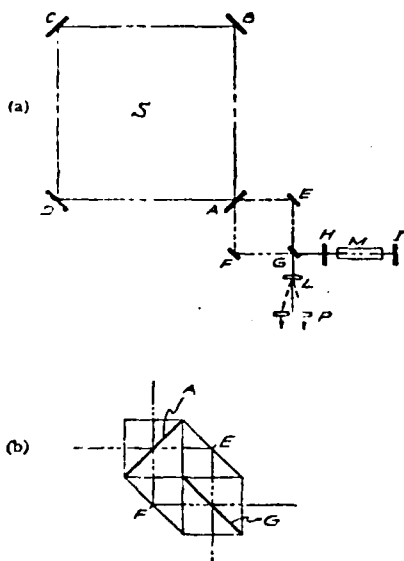
FIG. 3. (a) Schematic of circulatory multiple-beam interferometer with optical maser as outside light source. The resolution is instrument limited. (b) Prism assembly for auxiliary circuit of Fig. 3.
