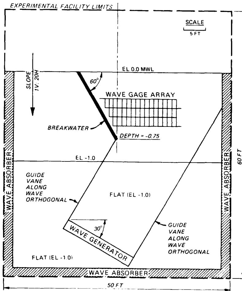
Figure 1. Experimental layout
