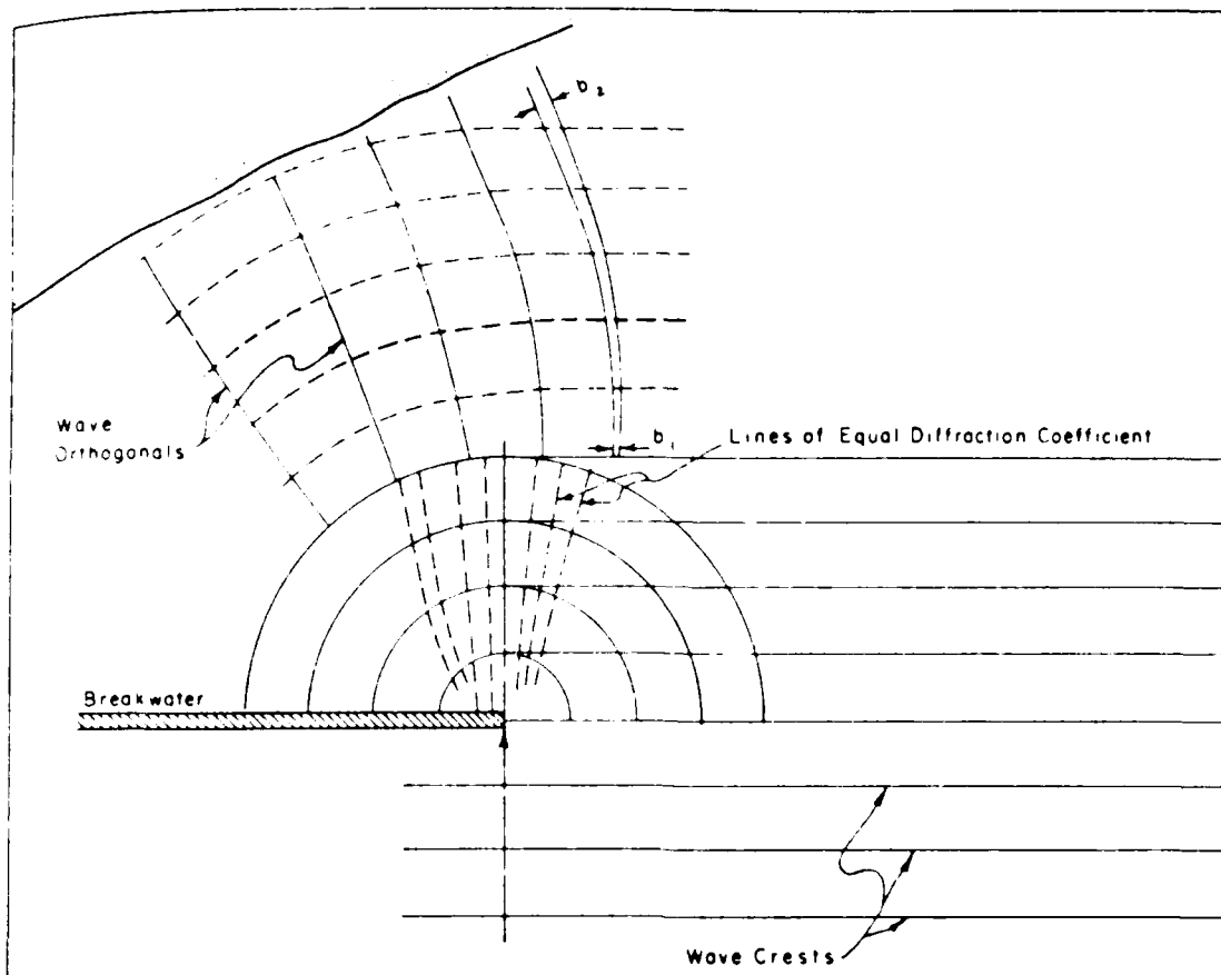
Figure 10. Graphical procedure for determining overall refraction and diffraction effects past a breakwater (after CERC 1977)
