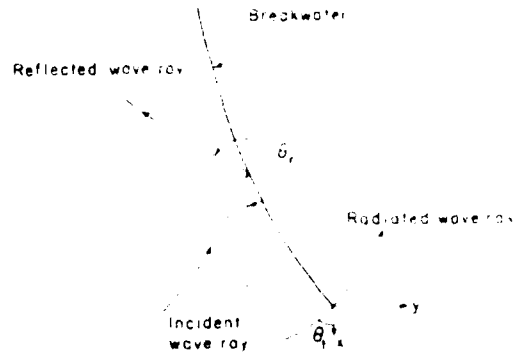
Figure 13. Definitive sketch, uniformly valid asymptotic theory, relation between incident wave angle and the reflected wave angle along the breakwater (Liu, Lozano, Pantazaras 1979)
