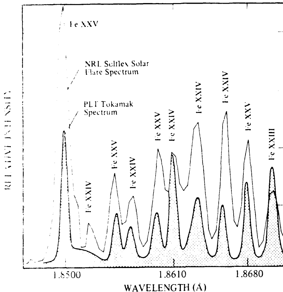
FIGURE 5.1 An x-ray emission spectrum of a solar flare obtained by a Naval Research Laboratory (NRL) instrument aboard satellite STP-78-1 compared with the spectrum of a plasma in the Princeton large tokamak. The spectral lines are associated with transitions in highly ionized iron (Fe XXIII, XXIV, and XXV, with 22, 23, and 24 electrons stripped off, respectively). To produce these ions requires an electron temperature in excess of 12 \times 10^6 K. For the spectra shown here, the flare temperature is 17 \times 10^6 K and the tokamak temperature is 20 \times 10^6 K. The resemblances are striking; the differences are due not to the slight difference in temperature but to the fact that the flare plasma is close to ionization equilibrium, while the tokamak plasma is still rapidly heating up. (Courtesy of NRL.)
