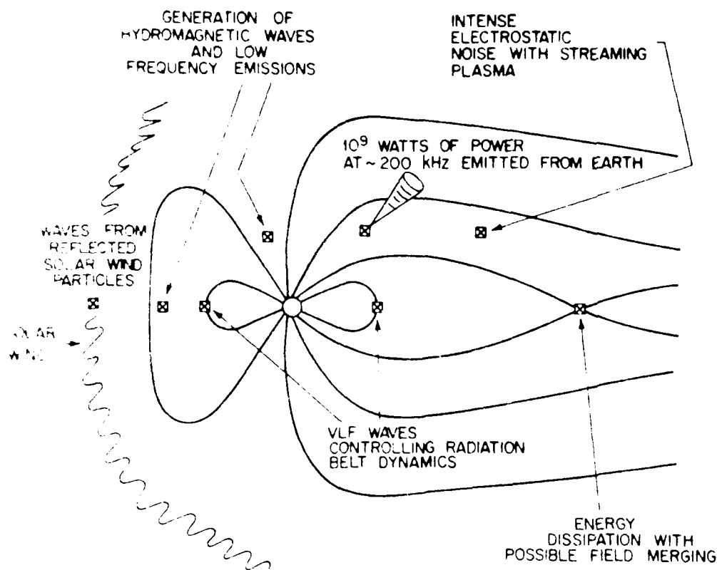
FIGURE 5.8. A schematic noon-midnight section of the earth's magnetosphere showing regions with significant plasma-wave activity. Compare with Figure 1.3 in order to identify the locations mentioned below.
