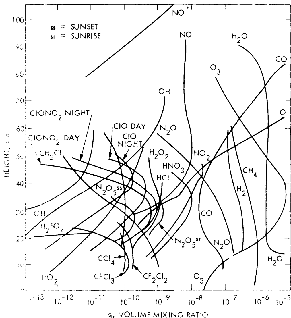
FIGURE 5-10 Altitude profiles of the concentration of minor constituent species in the middle atmosphere. (From the Report of the Science Definition Working Group, Upper Atmosphere Research Satellite, courtesy of the Jet Propulsion Laboratory, California Institute of Technology.)
