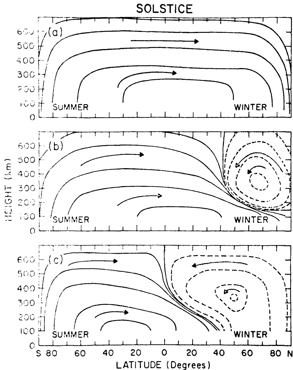
FIGURE 5.9 Diagrams of the mean meridional circulation in the thermosphere at the time of the winter solstice in the northern hemisphere, for three levels of auroral or geomagnetic activity. (Courtesy of R. G. Roble, NCAR.)
