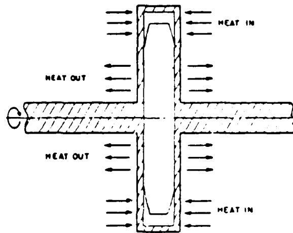
(f) Disk-Type
