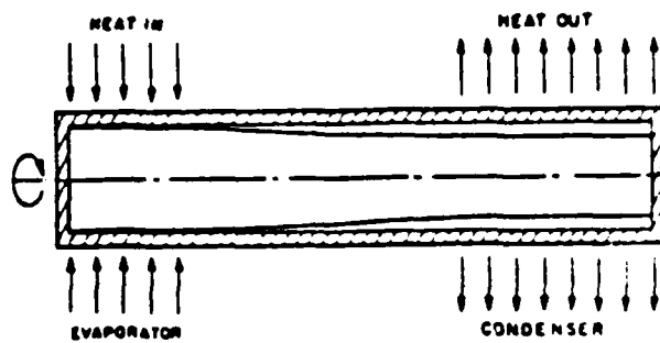
(a) Circular
