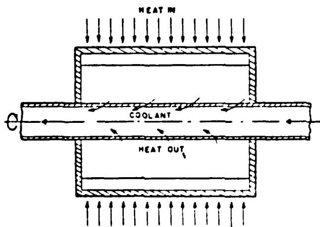
(e) Drum-Type
