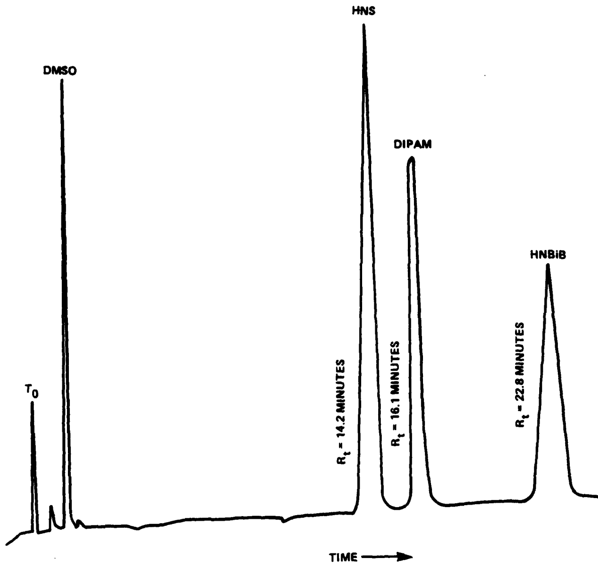
FIGURE 5. HPLC CHROMATOGRAM OF HNS, HNBIB, AND DIPAM
