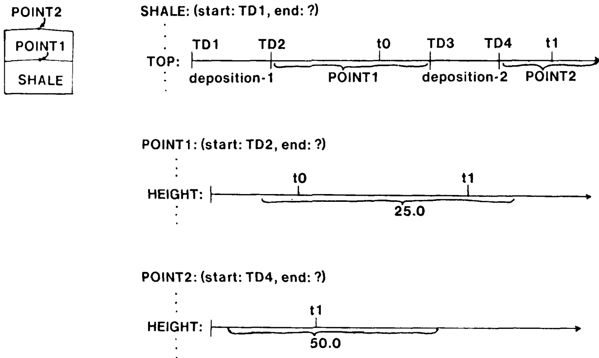
Fig. 12. History Representation after Deposition of More Shale
