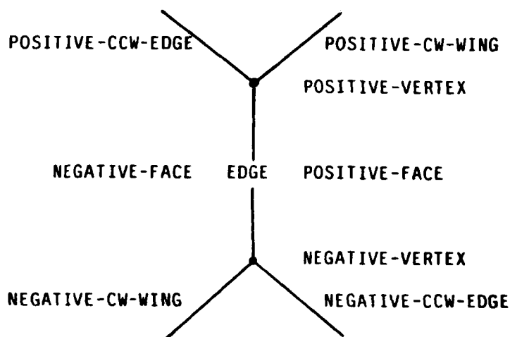
Fig. 15. The Wing-Edge Representation of an Edge
