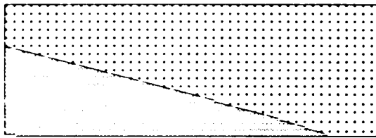
2. Intrude Granite
