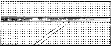
4. Deposit Sandstone-2
