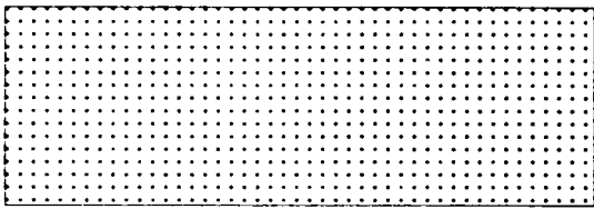
1. Deposit Sandstone
