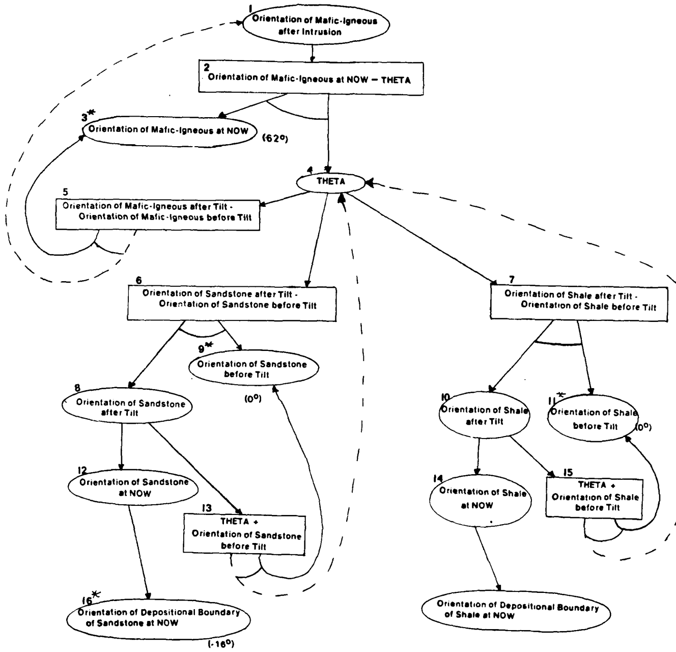
Fig. 8. Partial AND-OR Graph for Parameter Determination
