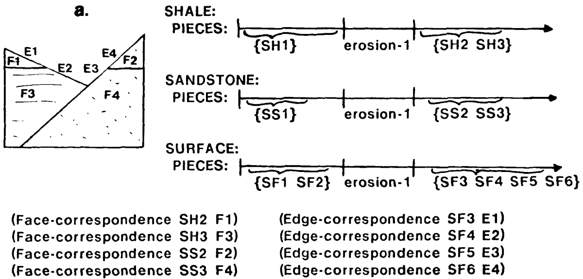
Fig. 27. Maintaining the Piece Structure When Manipulating Diagrams
