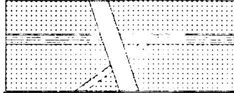
5. Intrude Granite-2
