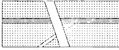
6. Uplift
