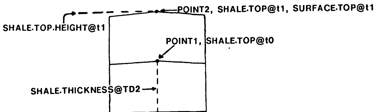
Fig. 14. @ Notation
