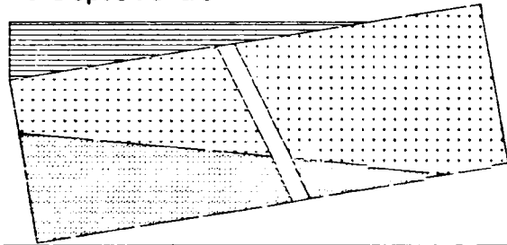
5. Deposit Shale
