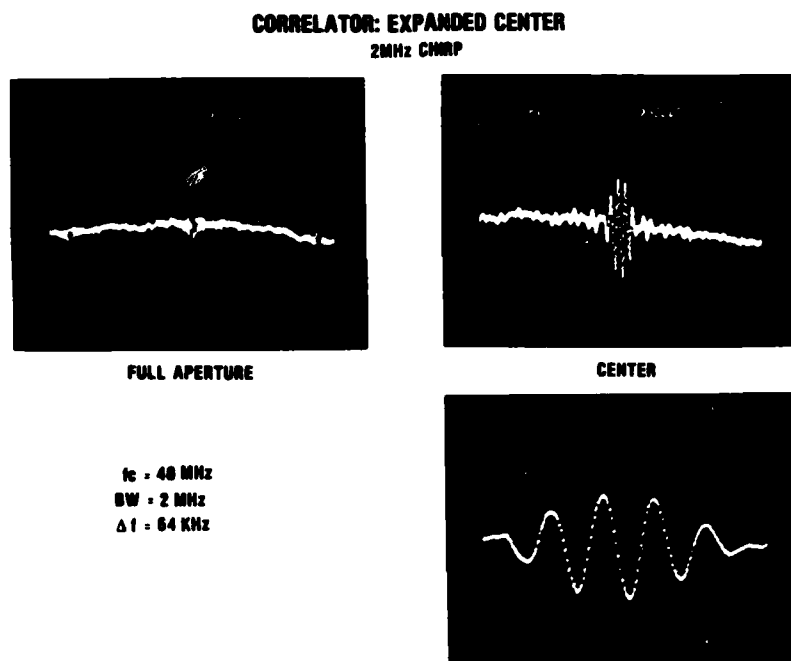
Figure 4. Output of the M = 10 correlator section for the same 2-MHz bandwidth chirp used in figure 3, with \Delta f = 64 \text{ kHz} . Shown is full aperture and the center 4 \mu\text{s} of correlation space. Center frequency of the chirp f_c is 40 MHz.
