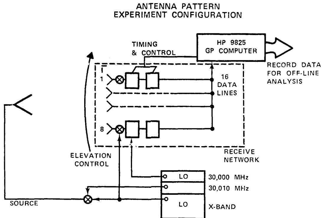
Figure 3. Block diagram of pattern recording equipment and receiver test network.
