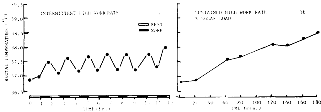
FIGURE 5. Average Rectal Temperatures of M1 Tank Crewmen During 12 hr. (5a) and 180 min. Engineering Design Tests of the M1E1.
