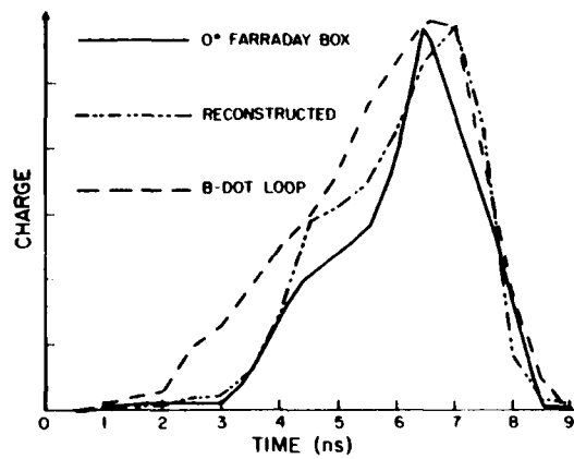
Fig. 11. Charge-vs-time.
